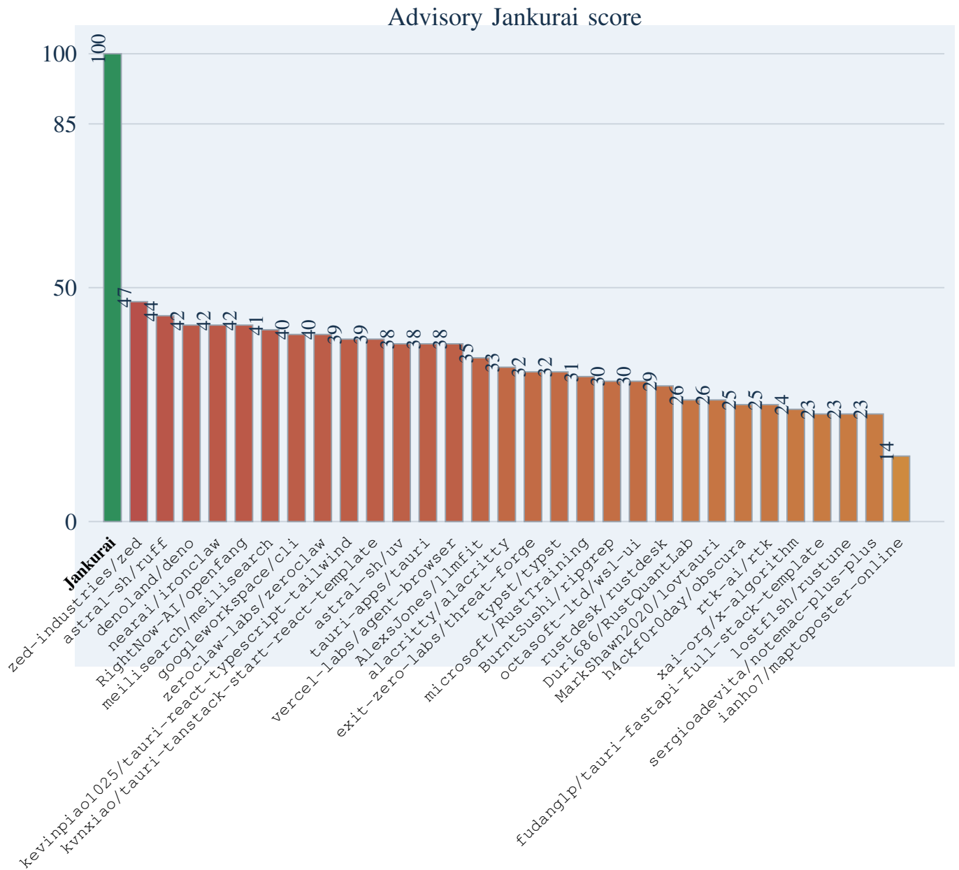
Fig. 5. Advisory public-repository score ranking with the Jankurai repository baseline included. Bars are sorted by score; color moves from red through amber to green as scores approach the merge-witness-ready band.
