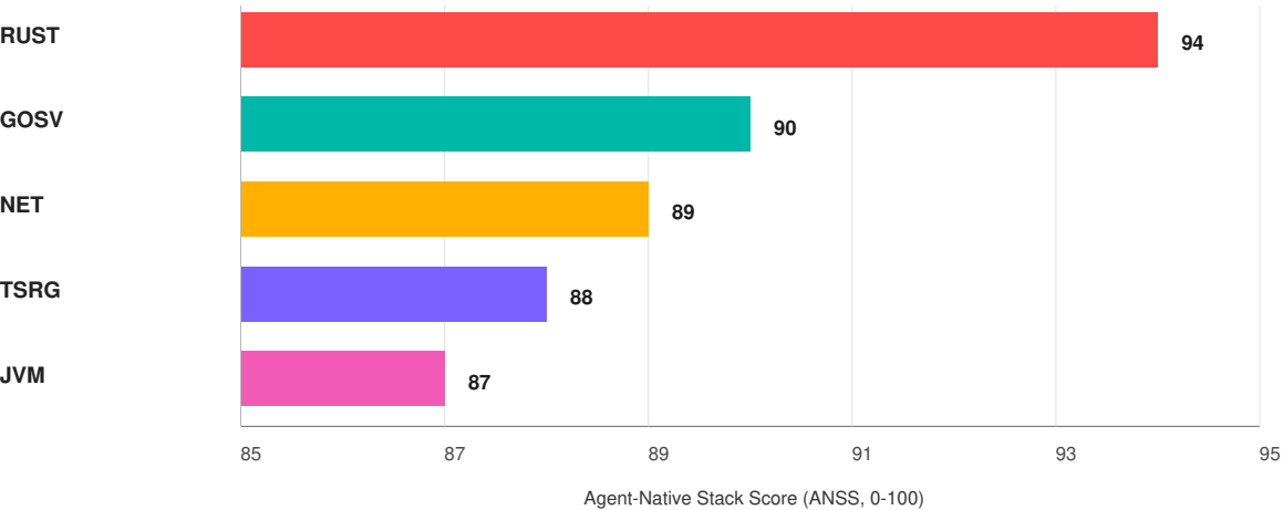
Fig. 2. Top-five stack ranking by Agent-Native Stack Score (ANSS), the weighted jankurai 100-point rubric. The figure is a zoomed comparison of close contenders; Table VIII gives the absolute scores. Labels: RUST = Rust core, GOSV = Go services, NET = C#/.NET, TSRG = TypeScript product plane with Rust/Go compute cells, and JVM = Kotlin/Java. All entries assume TypeScript/React/Vite product surface and PostgreSQL durable truth; streaming buses are workload-specific additions.
