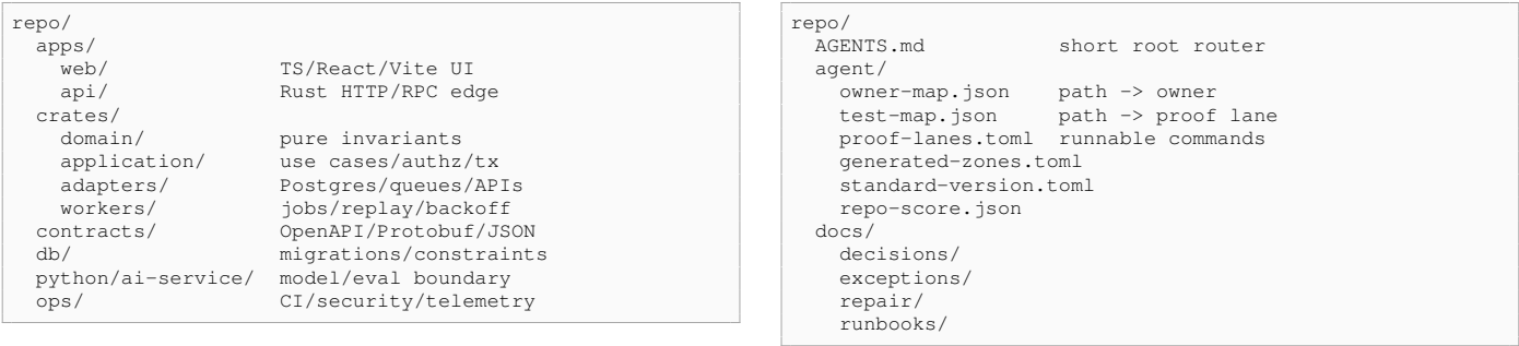
Fig. 3. Ownership spine and agent-control spine for the default stack.
