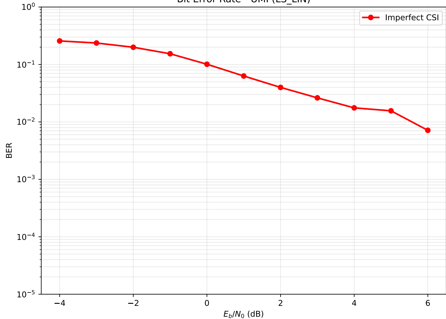
Bit Error Rate - UMI (LS_LIN)
