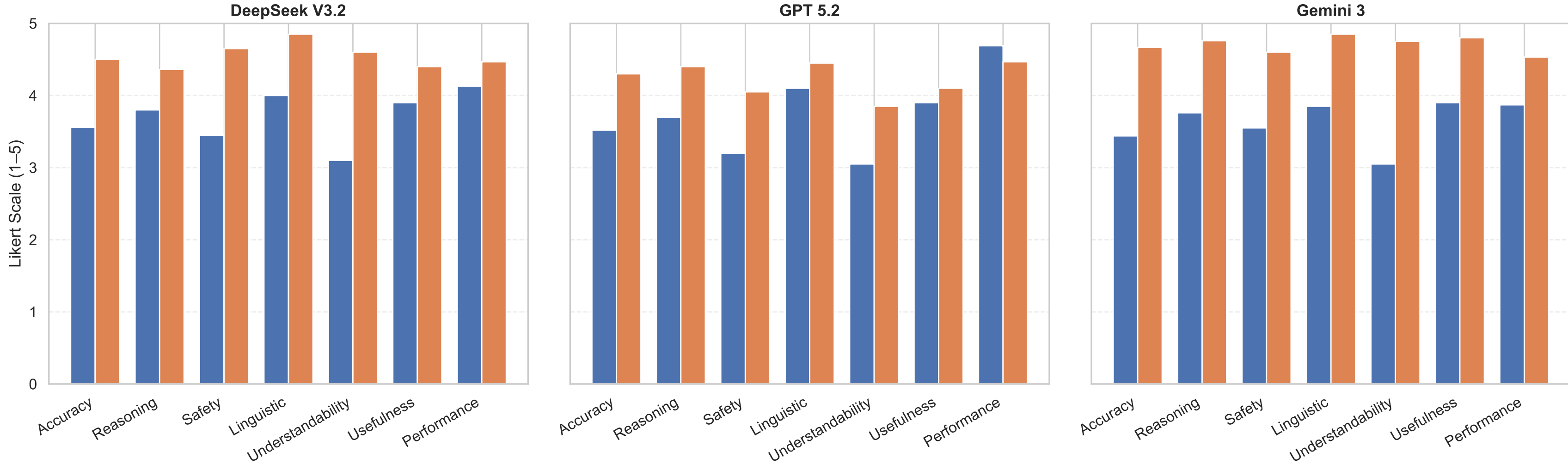
Paired Validation (Model × Domain): MELMA-W vs Human Evaluators
