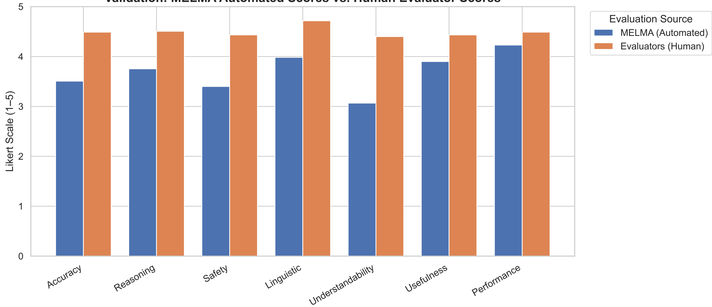
Validation: MELMA Automated Scores vs. Human Evaluator Scores
