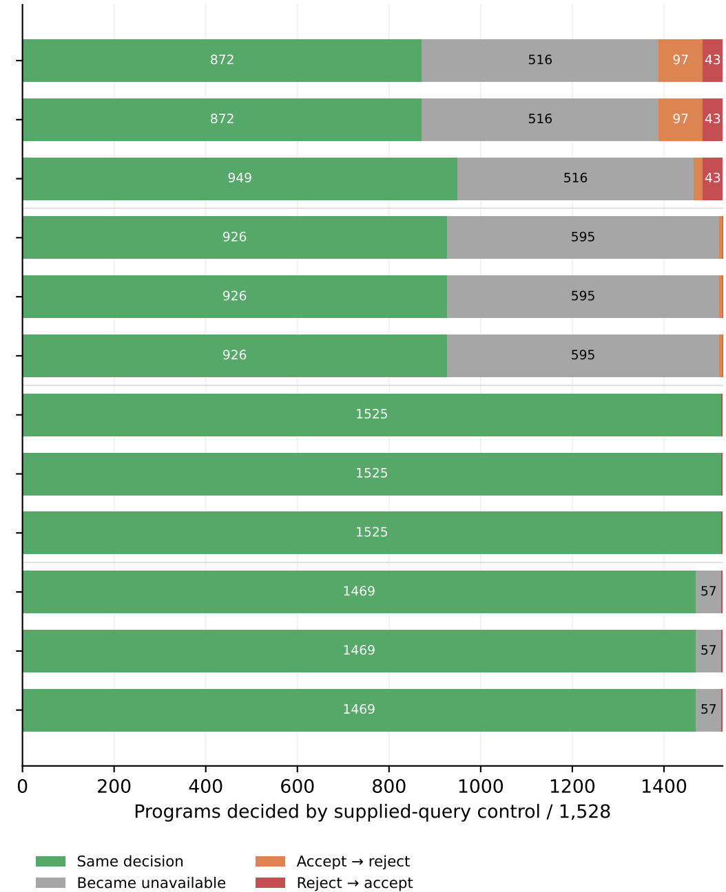
B. Downstream decision preservation
