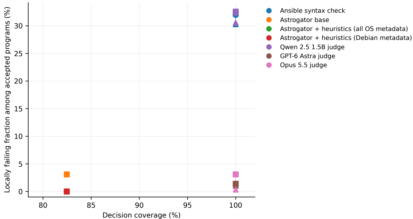
Coverage and accepted-program risk under label sensitivity
