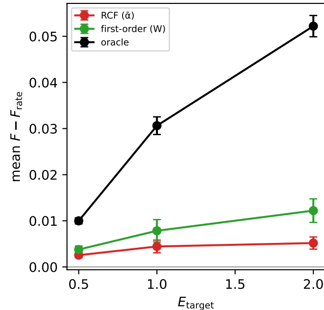
Random ensemble
