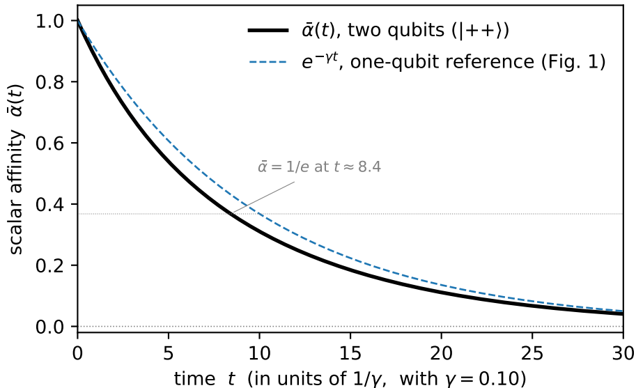
Scalar affinity under independent dephasing of |++\rangle
