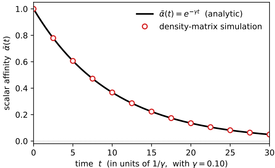
Single-qubit affinity decay: |+\rangle under Markovian dephasing
