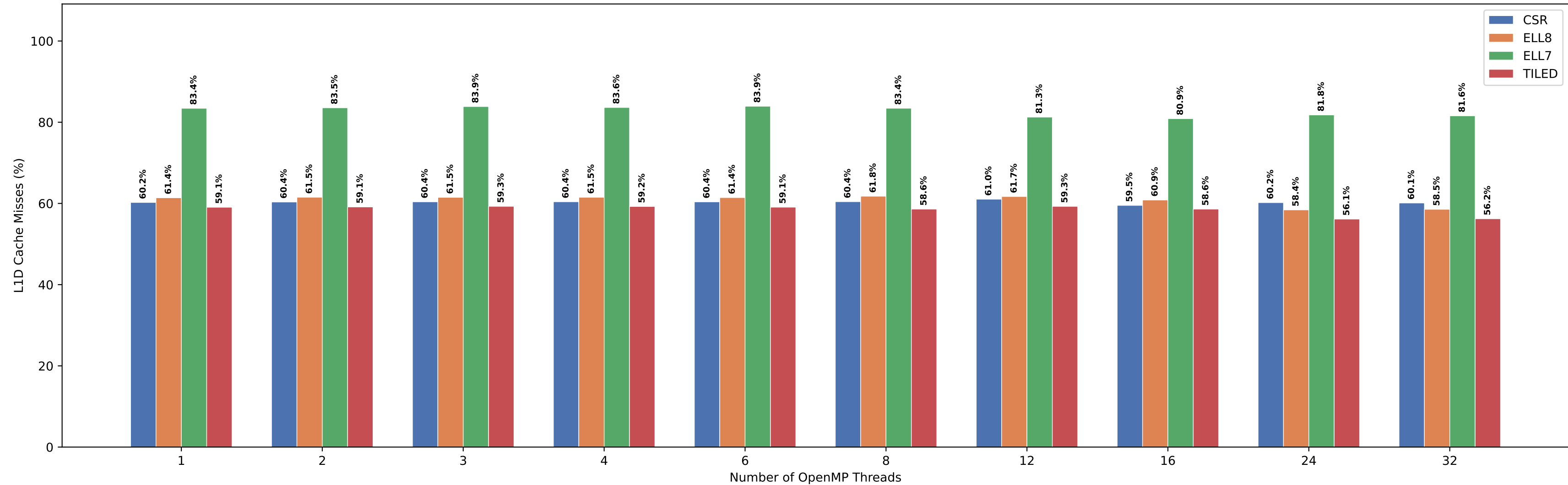
SpMV L1D Cache Misses — Matrix 200x200x200
