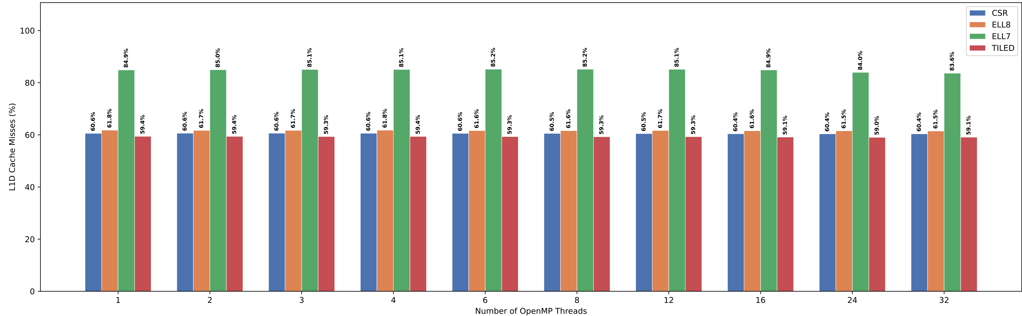
SpMV L1D Cache Misses — Matrix 250x250x250
