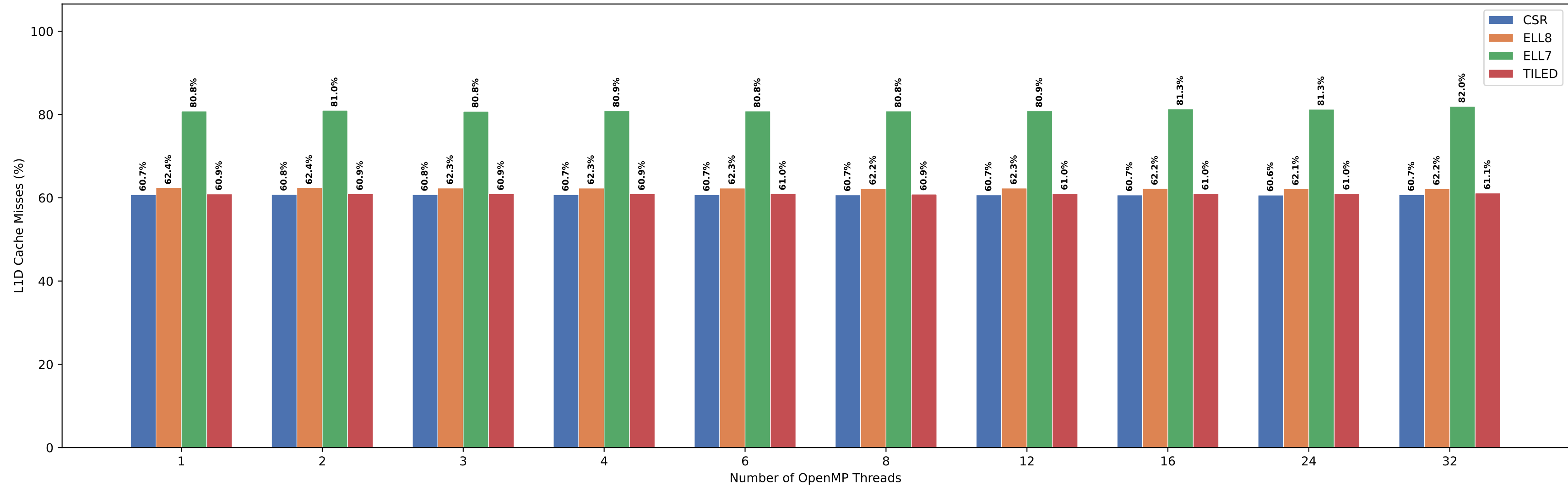
SpMV L1D Cache Misses — Matrix 300x300x300
