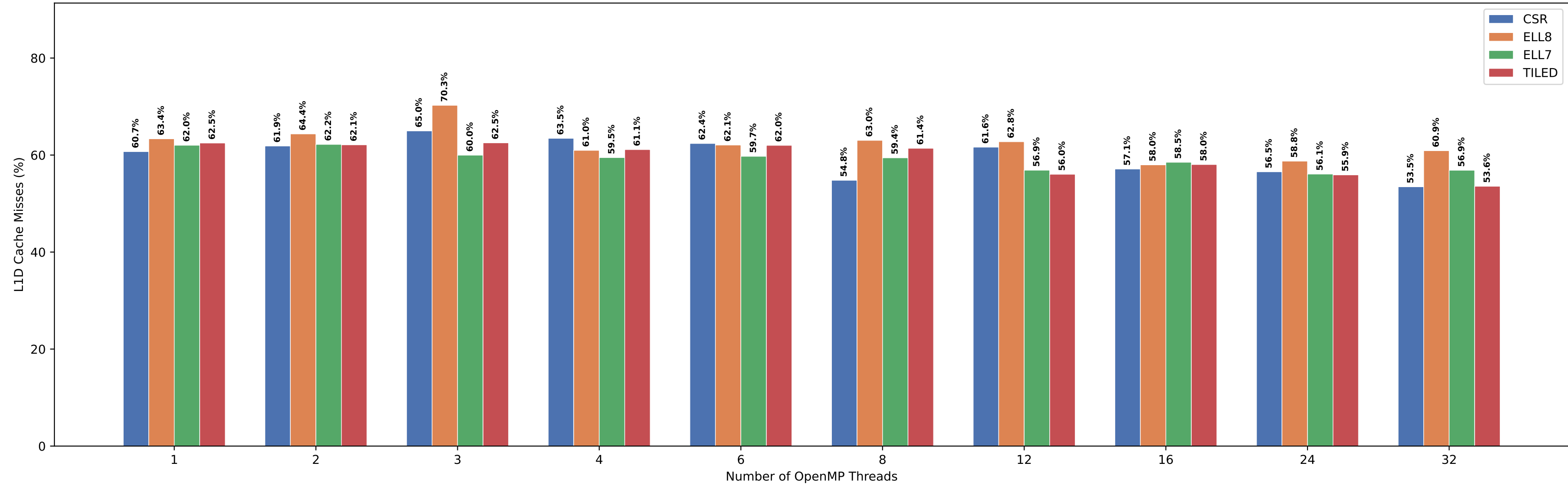
SpMV L1D Cache Misses — Matrix 50x50x50
