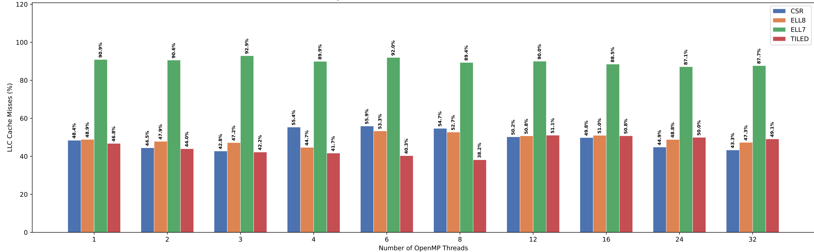
SpMV LLC Cache Misses — Matrix 100x100x100
