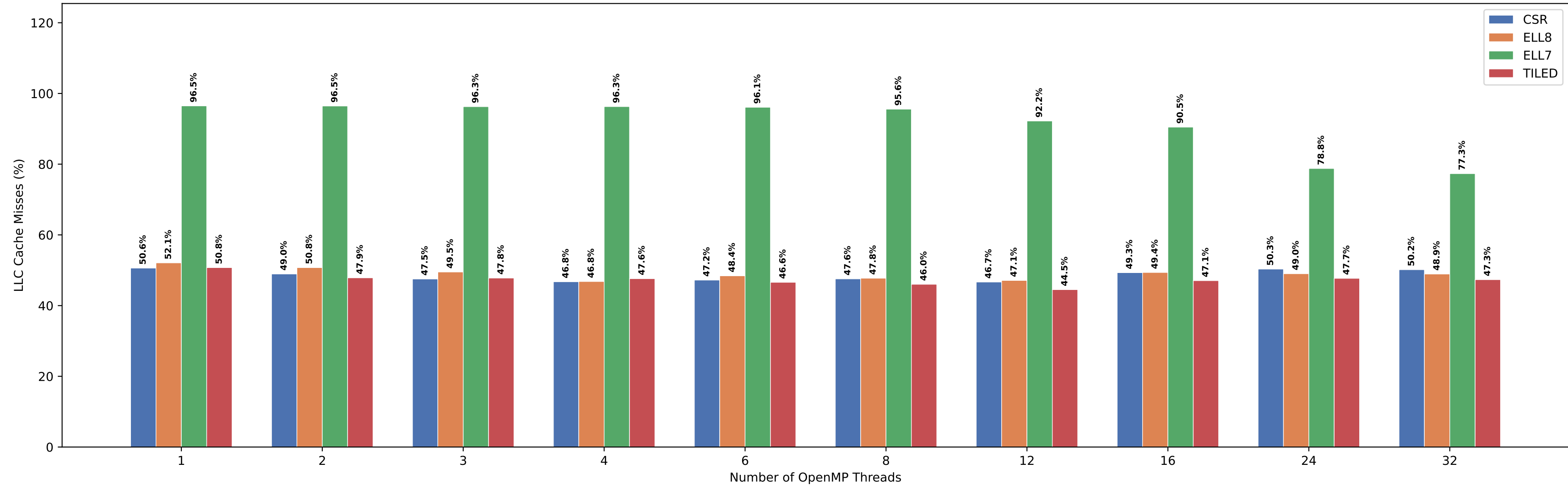
SpMV LLC Cache Misses — Matrix 150x150x150
