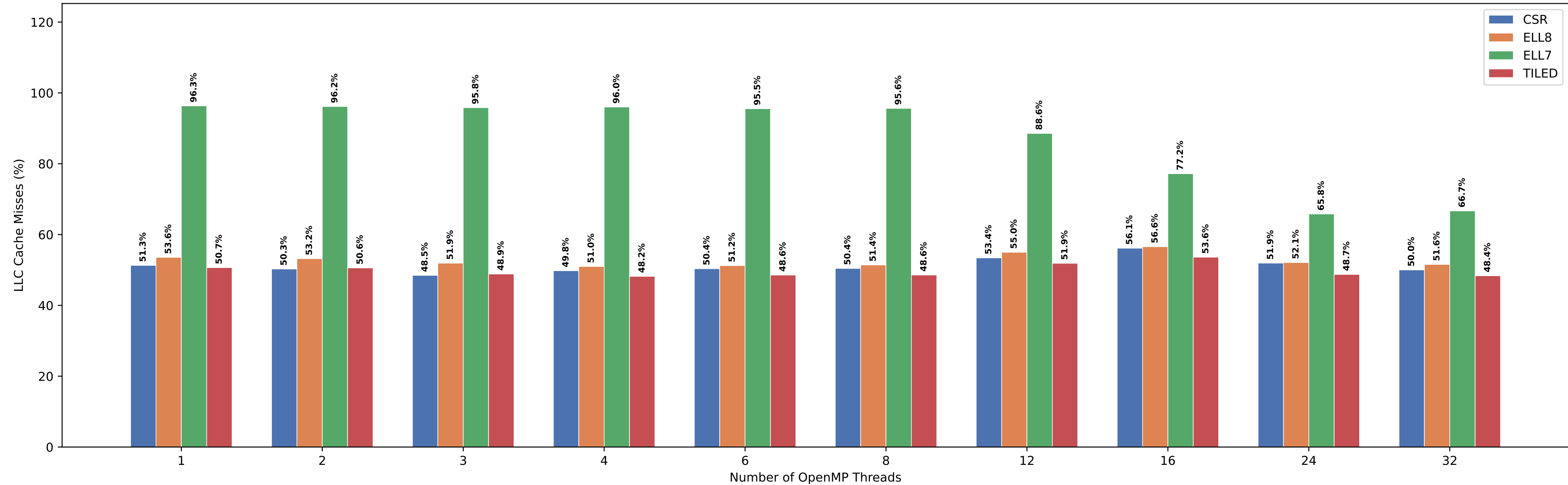
SpMV LLC Cache Misses — Matrix 200x200x200
