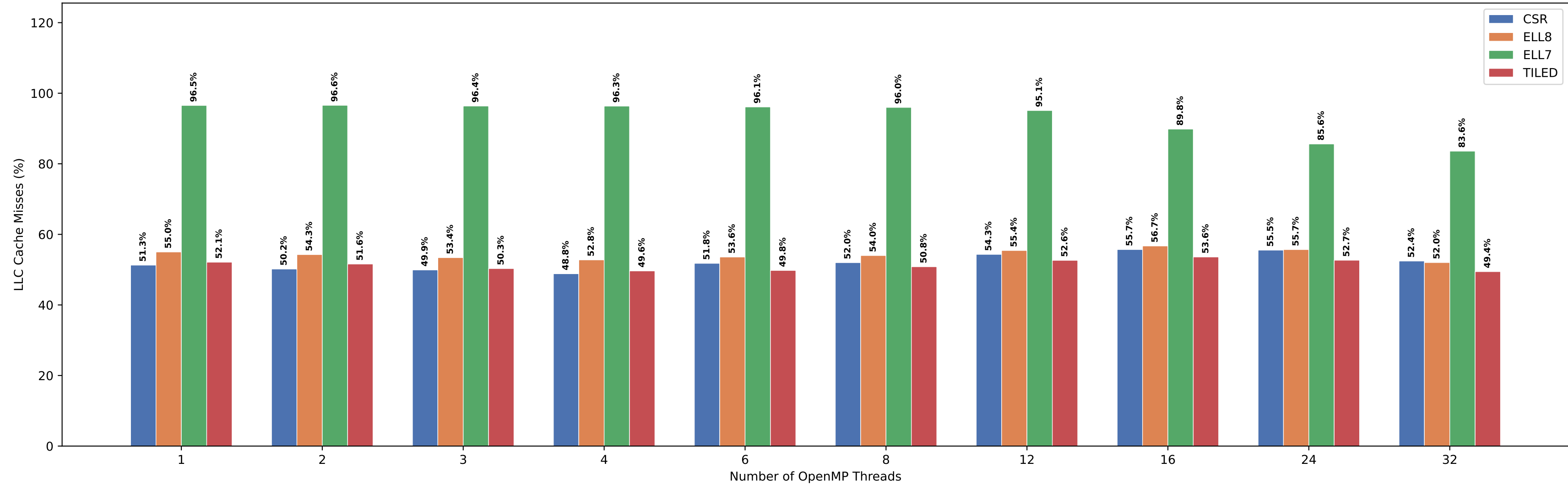
SpMV LLC Cache Misses — Matrix 250x250x250
