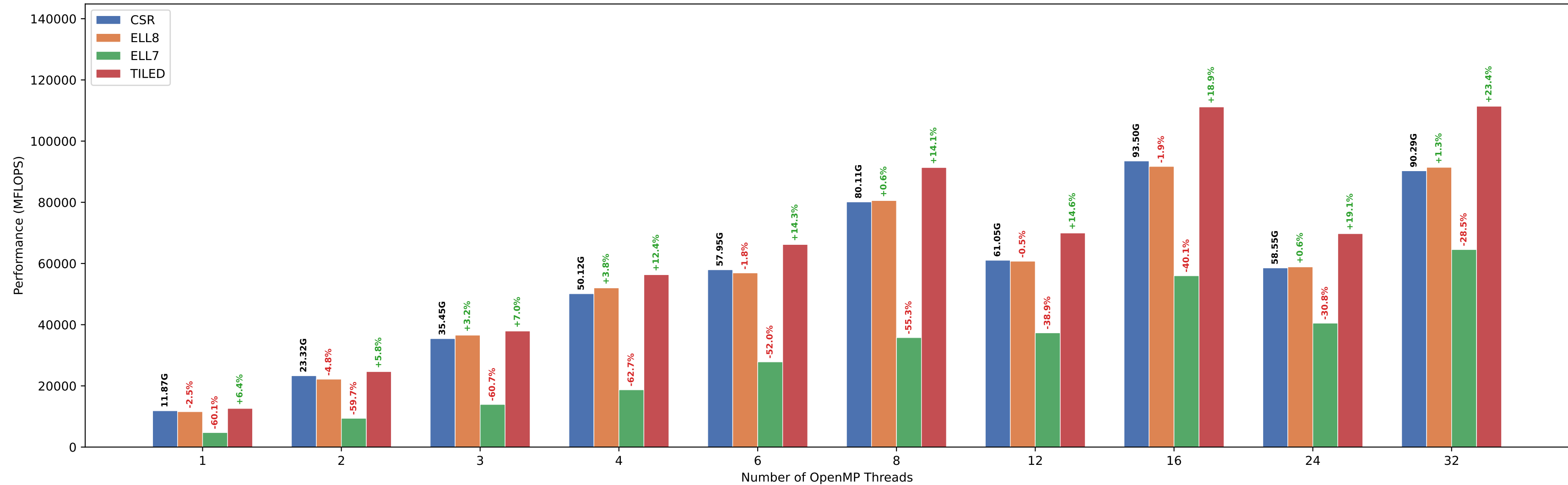
SpMV MFLOPS — Matrix 150x150x150
