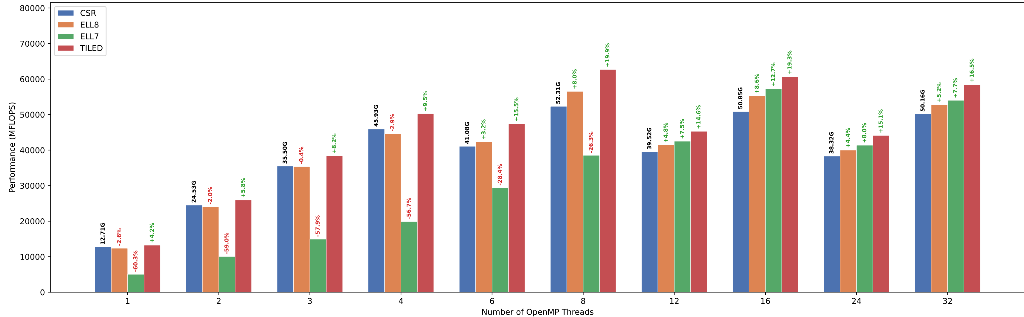
SpMV MFLOPS — Matrix 300x300x300
