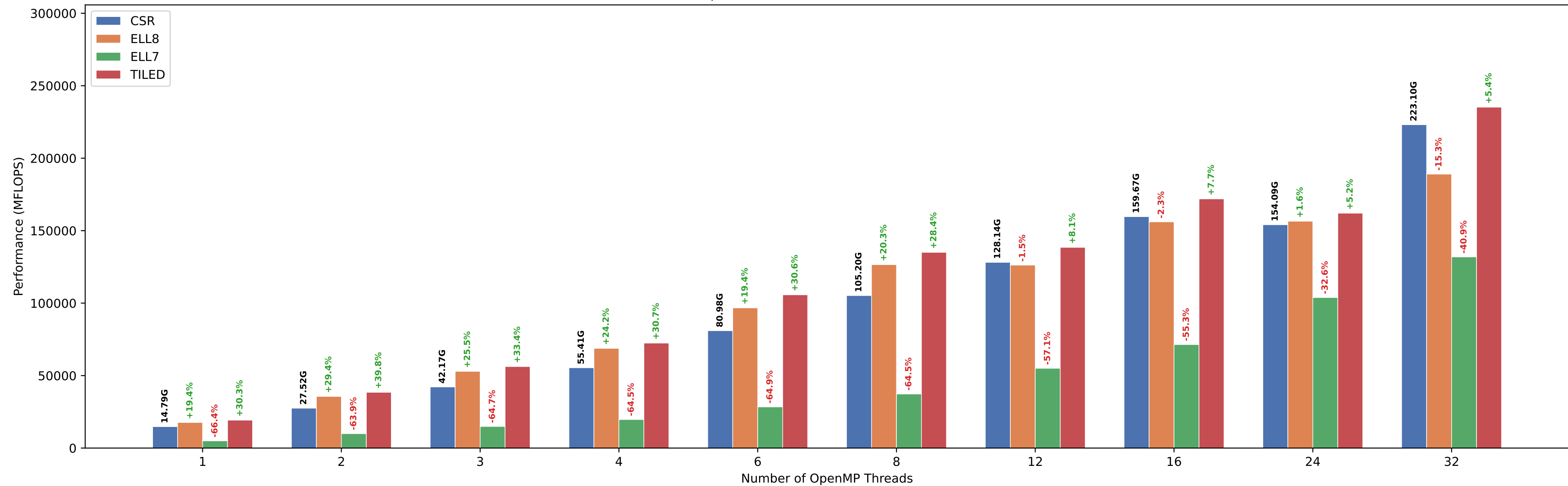
SpMV MFLOPS — Matrix 50x50x50
