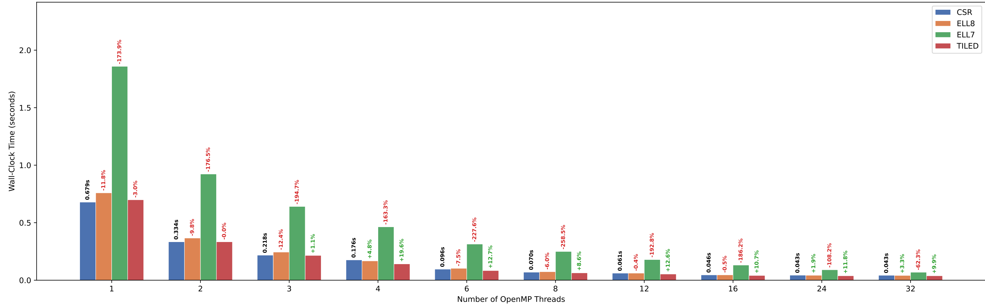
SpMV Wall-Clock Time — Matrix 100x100x100
