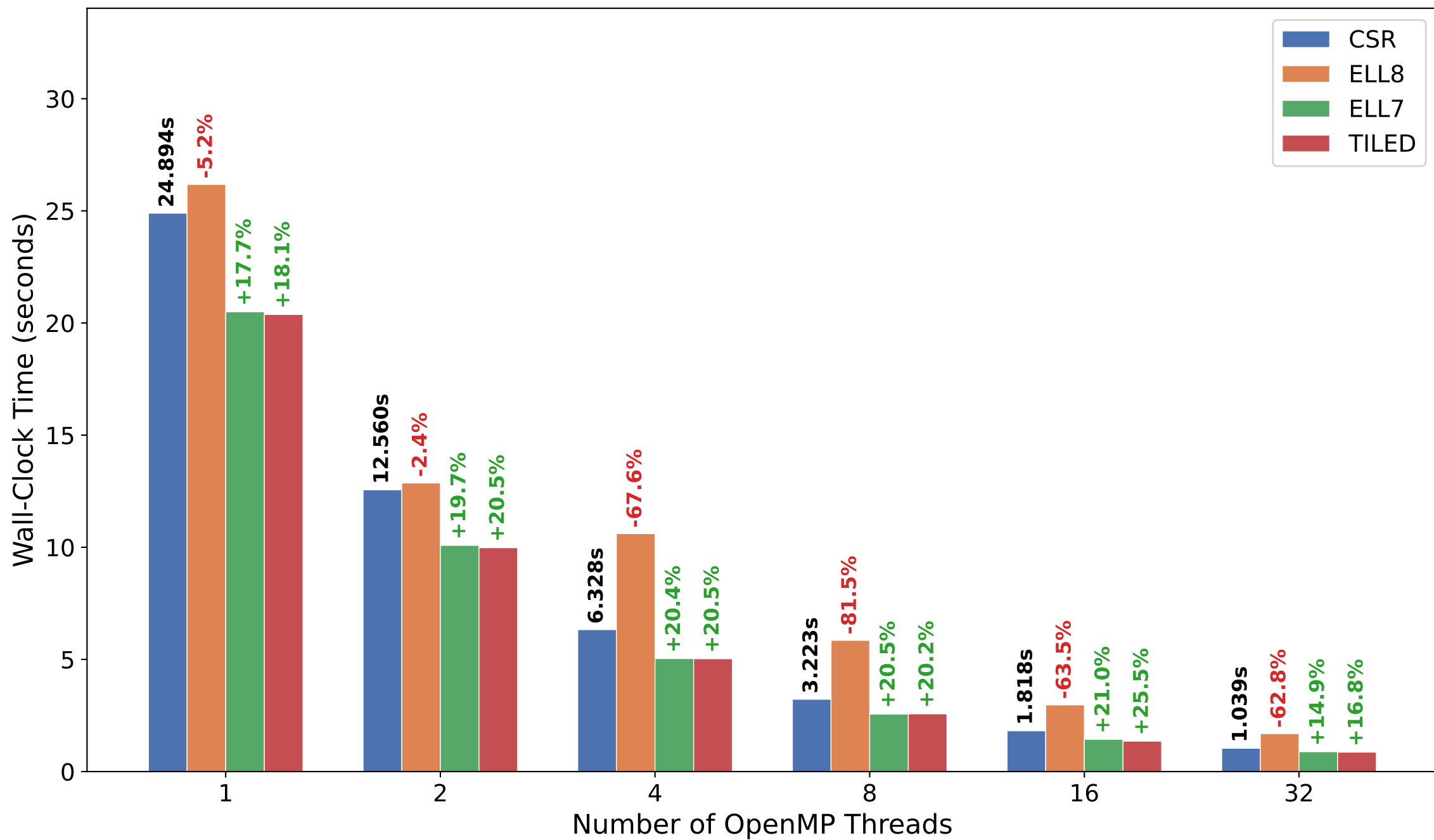
SpMV Wall-Clock Time — Matrix 250x250x250
