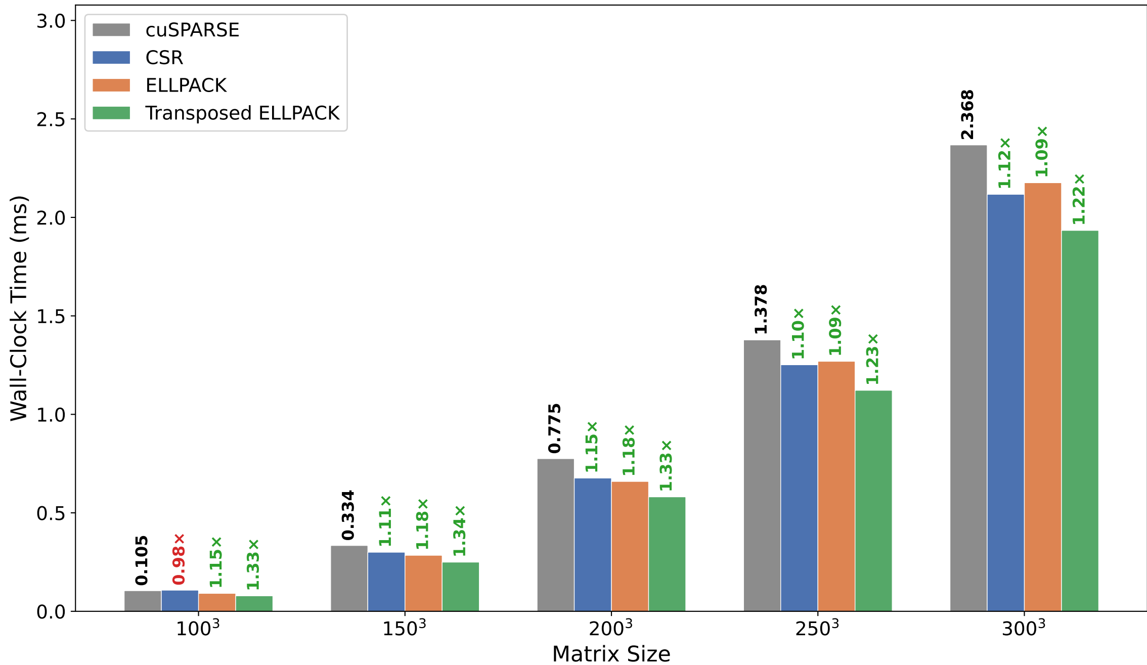
GPU SpMV Performance — Polaris (NVIDIA A100)
