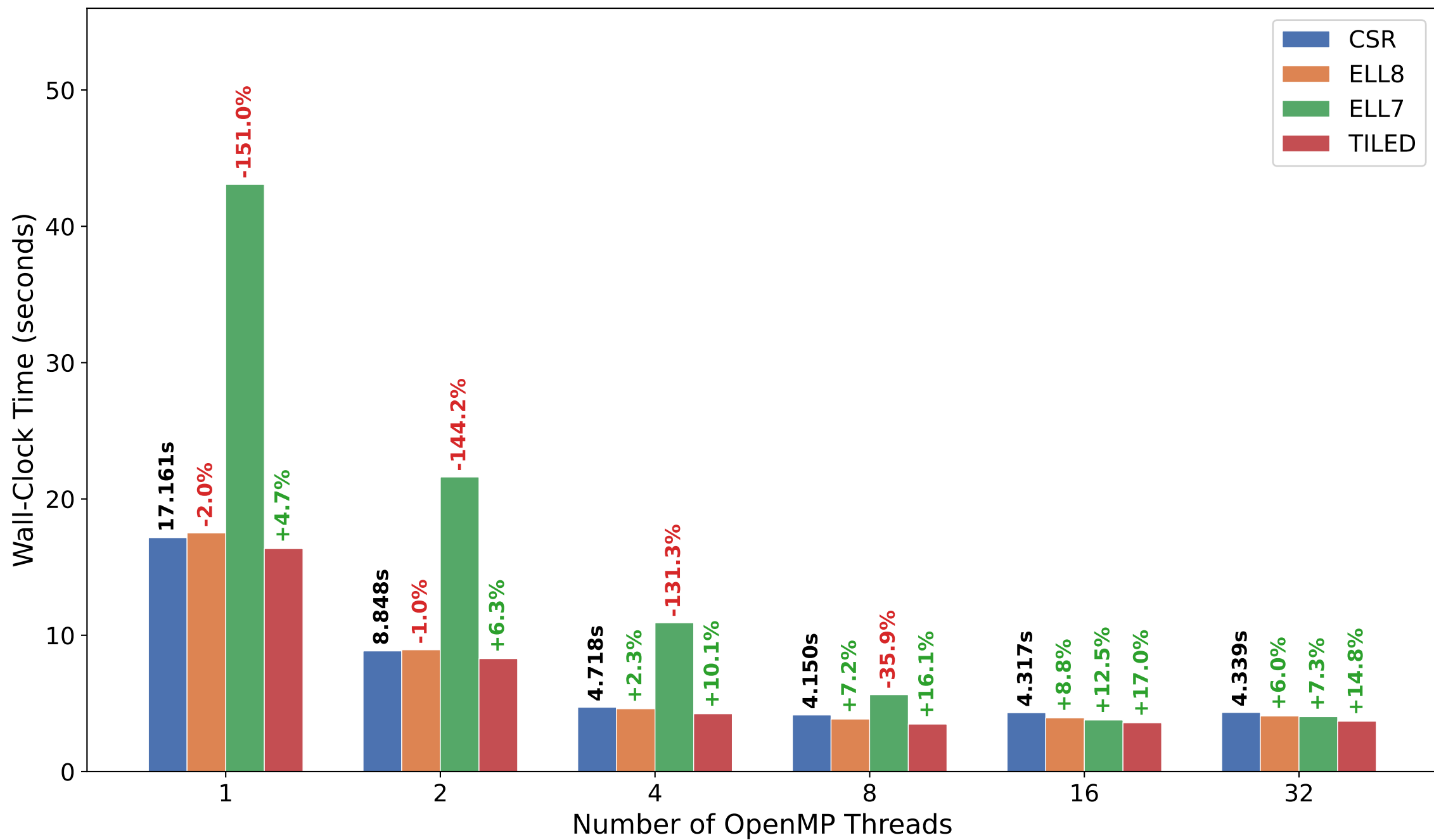
SpMV Wall-Clock Time — Matrix 300x300x300
