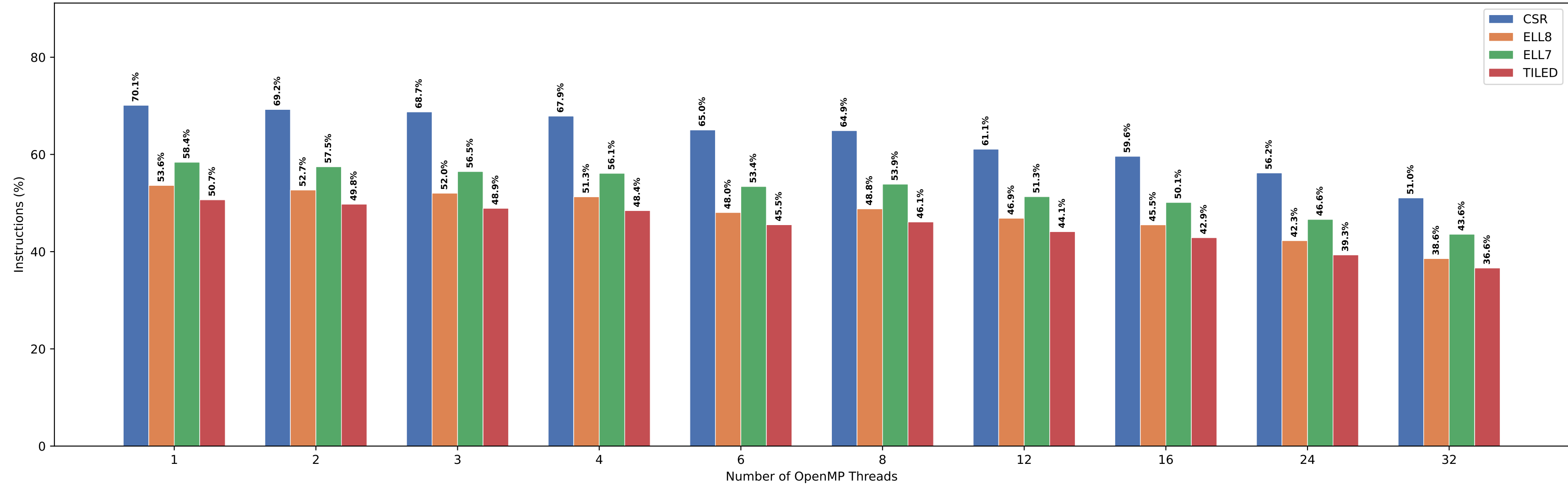
SpMV Instructions — Matrix 200x200x200
