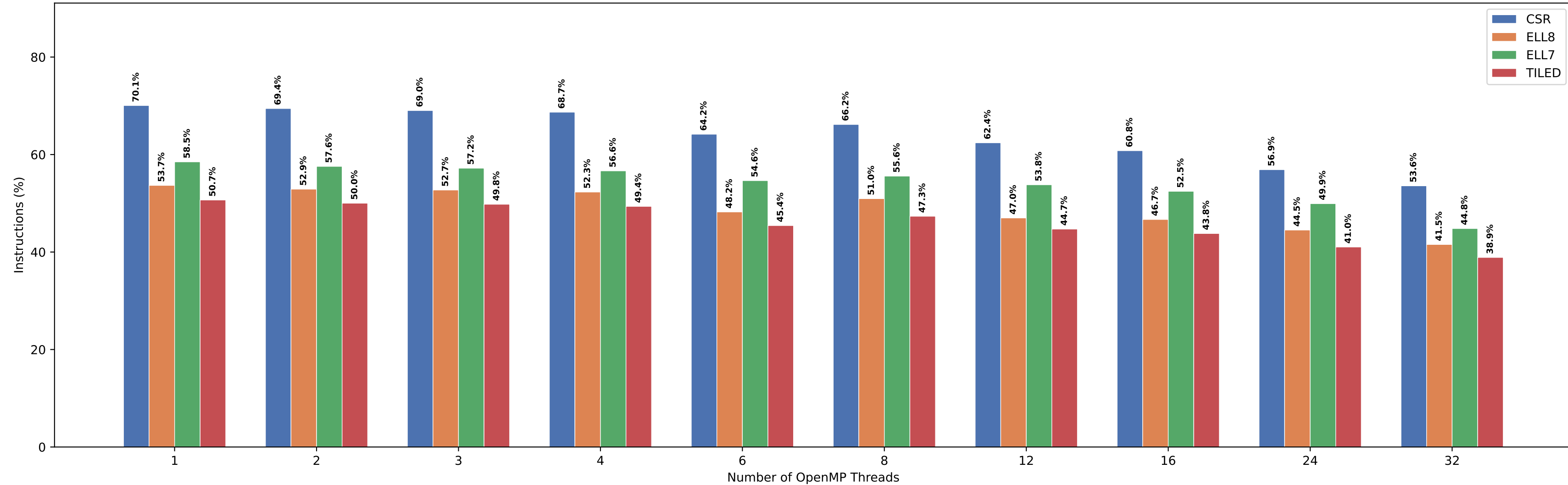
SpMV Instructions — Matrix 250x250x250
