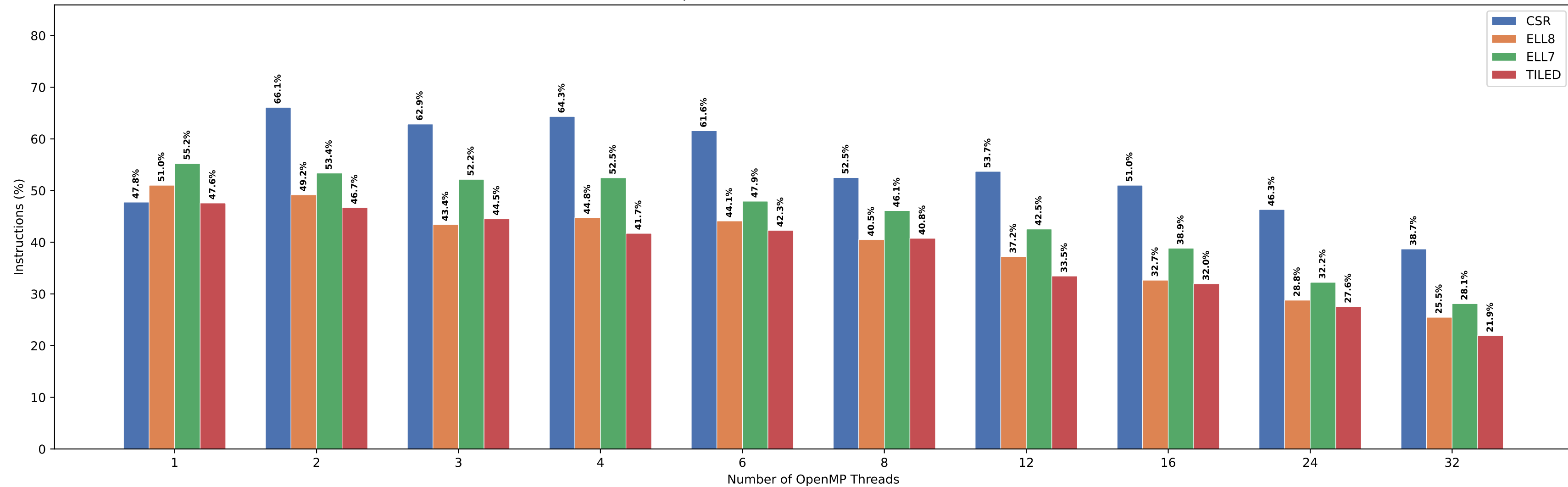
SpMV Instructions — Matrix 50x50x50
