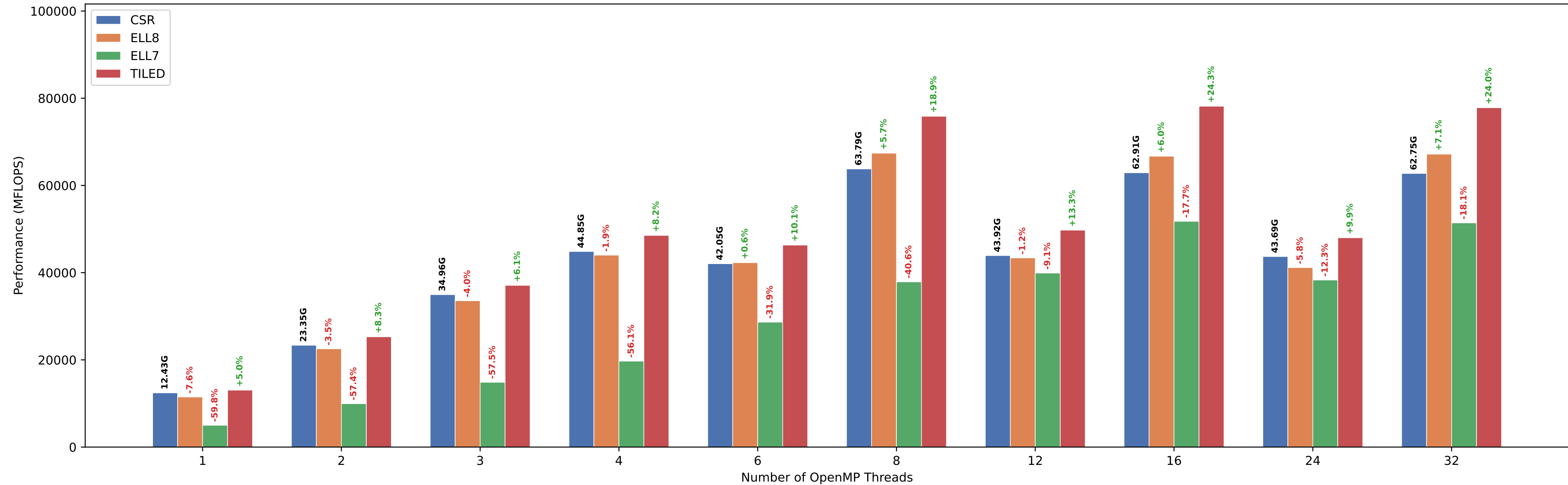
SpMV MFLOPS — Matrix 200x200x200
