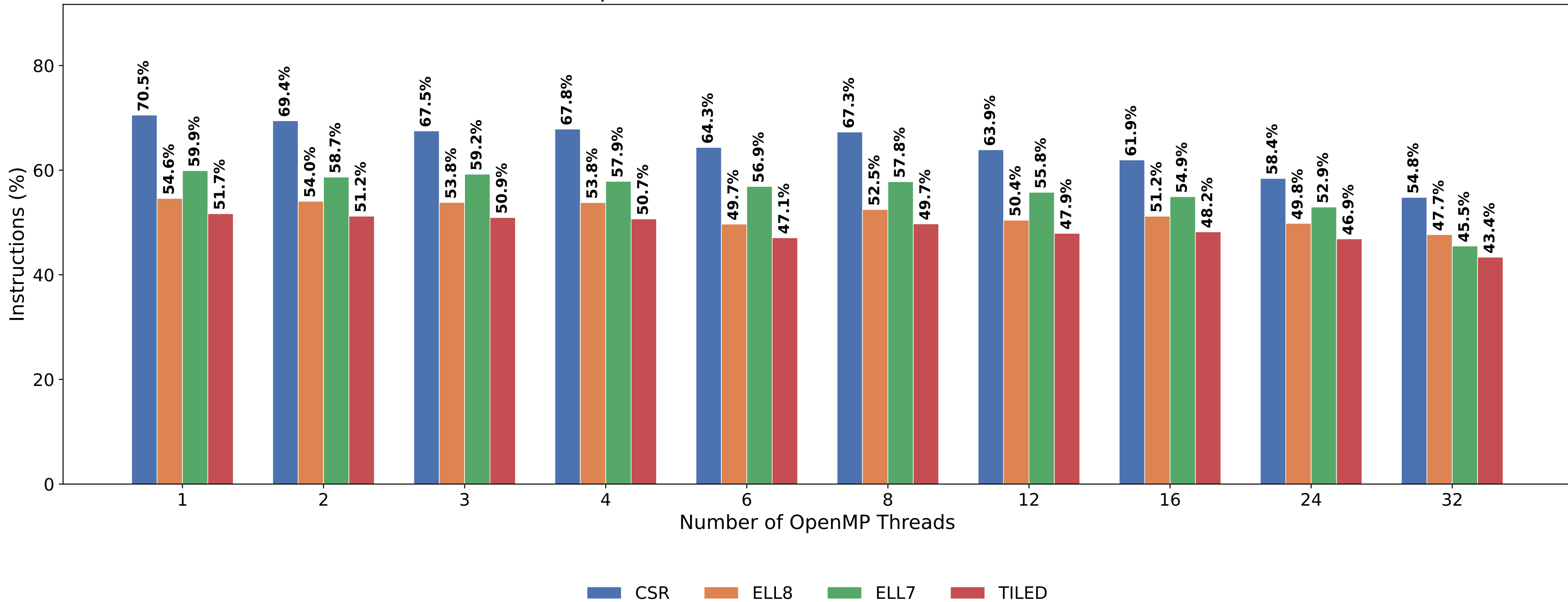
SpMV Instructions — Matrix 300x300x300
