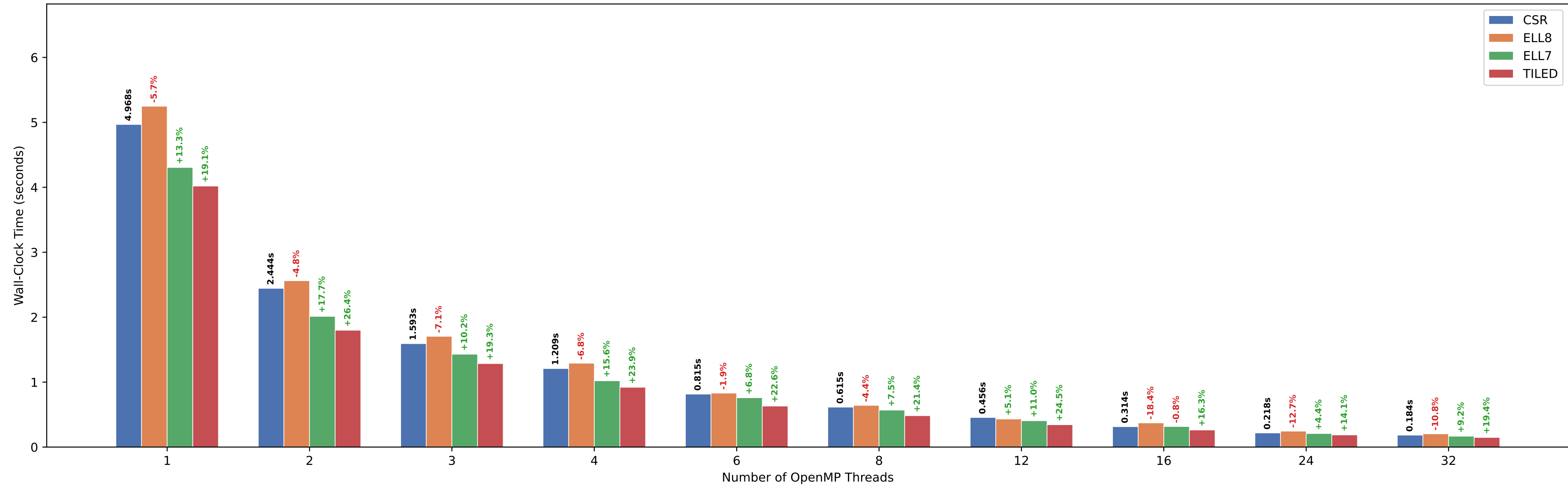
SpMV Wall-Clock Time — Matrix 150x150x150
