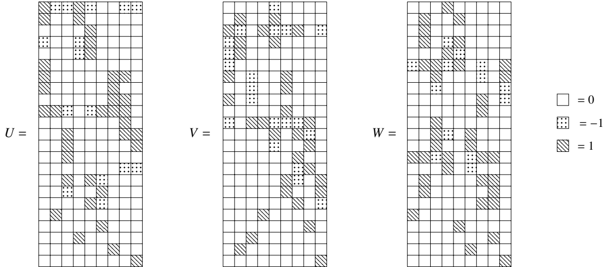
Fig. 8: Illustration of the matrices U , V , and W that constitute Laderman's rank-23 scheme for multiplying 3 \times 3 matrices [31]. These specific matrices U , V , and W were taken from the Laderman scheme provided by [4].
