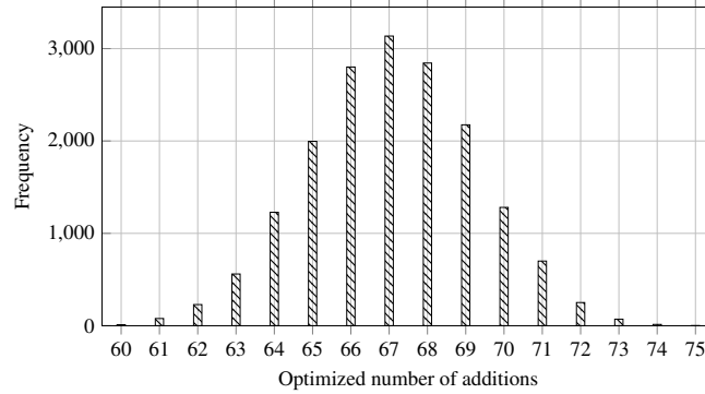
Fig. 34: For each Strassen-type matrix-matrix multiplication scheme from the dataset described in Section 3.1, the figure counts the total number of additions required to compute the three linear parts U, V , and W , see equation (2.3), after optimization by our framework. All instances were run on a single core on an Intel Xeon E5-2660 v3 CPU model, and each SLP instance was given a time limit of 4.8 seconds.
