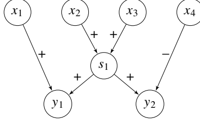
Fig. 2: Illustration of how we can save additions when computing the matrix-vector product Gx shown in equation (2.7). Any node except for x_1, x_2, x_3, x_4 represent the sum induced by the incoming edges. Edges marked with a "+" indicate addition of the source node, and those marked with a "-" indicate addition of the negated source node.
