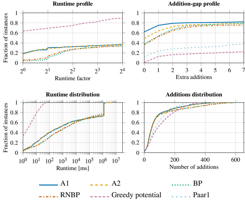
Fig. 32: Comparison of the six heuristics on the Bernoulli dataset. No preprocessing or postprocessing was applied. We remark that the Paar1 heuristic took 0 milliseconds (we round to nearest millisecond) on most data points, hence its missing representation on the runtime plots. All instances were run on a single core on an Intel Xeon E5-2660 v3 CPU model, and the time limit given was 1200 seconds per instance of SLP we solve.
