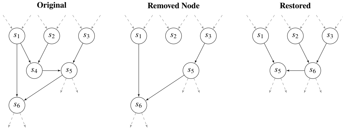
Fig. 42: Imagined DAG representation of the rule denoted R7 in [8]. The dashed edges represent possible involvement from outside the explicit part of the DAG we're looking at.
