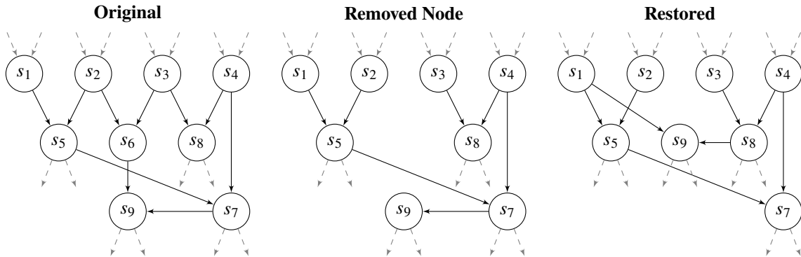
Fig. 45: DAG representation of the reduction not induced by any of the 11 preceding rules proposed in [8], but which our reduction method does successfully reduce. Note that s_6 is not used outside this part of our DAG. The dashed edges represent possible involvement from outside the explicit part of the DAG we're looking at.
