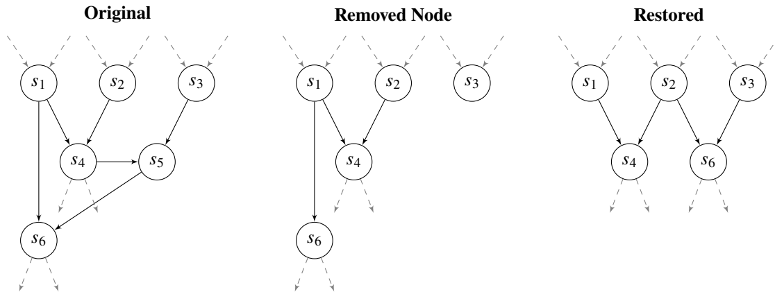
Fig. 41: DAG representation of the rule denoted R6 in [8]. The dashed edges represent possible involvement from outside the explicit part of the DAG we're looking at.
