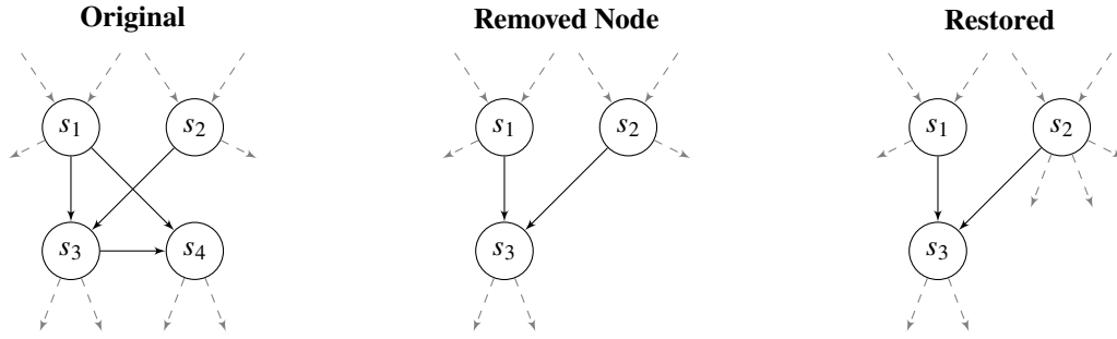
Fig. 36: DAG representation of the rule denoted R1 in [8]. The dashed edges represent possible involvement from outside the explicit part of the DAG we're looking at.
