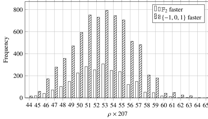
Fig. 26: Distribution over the schemes in the dataset described in Section 3.1 for which the \mathbb{F}_2 extension of the greedy potential method outperformed the corresponding ternary greedy potential method described in Section 4.2.2. \rho denotes the density, i.e. number of non-zero entries over the total number of entries. All matrices in the schemes in our dataset consist of 207 = 23 \cdot 9 entries, hence making the scaled density \rho \cdot 207 integer valued. When the time required to compute a scheme was equal, we add an entry for that frequency to both bars. The data used here is derived from that which was used to compute Figure 25, i.e. it was not computed anew.
