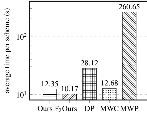
Fig. 25: Speed comparison between implementations of the greedy potential heuristic described in Section 4, ‘DP’ is the implementation by [49], ‘MWC’ is the C-implementation provided by [25], and ‘MWP’ the Python implementation also provided by [25]. The comparison was done on the 3 \times 3 matrix multiplication scheme dataset provided by [4], see Section 3.1. Note that our \mathbb{F}_2 implementation is working over \mathbb{F}_2 , while all other implementations work over \{-1, 0, 1\} . Also note that ‘MWP’ did not go through the whole dataset within the 72 hours of compute we allotted to it, while the other methods did manage to go through the whole dataset. All runs were allotted a total of 72 hours on a single core on an intel Xeon E5-2660 v3 CPU to go through the entire dataset.
