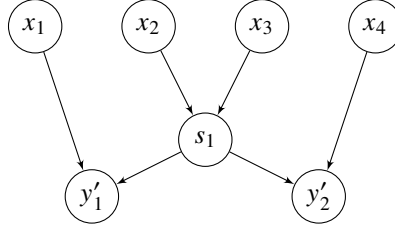
Fig. 4: DAG formulation of addition scheme for G' as it is defined in equation (2.15).
