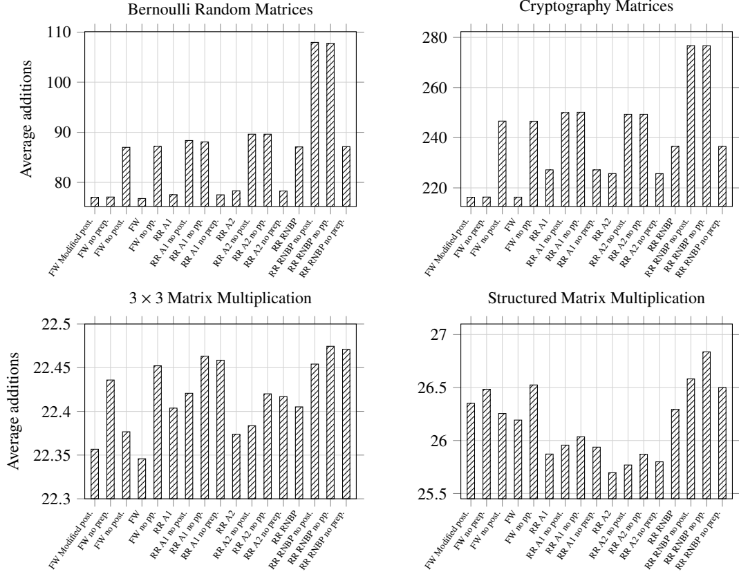
Fig. 33: Average number of additions found by each method on the Bernoulli, Cryptography, 3 \times 3 matrix multiplication, and structured datasets. Each data point of the Bernoulli dataset is run for 350 seconds, each data point in the Cryptography dataset is run for 4000 seconds, each data point in the 3 \times 3 matrix multiplication dataset is run for 4.8 seconds, and each data point in the structured matrix multiplication dataset is run for 350 seconds. The method FW Modified post. is the full framework with both preprocessing and postprocessing, where the postprocessing is as described in Section 4.3. The method FW no prep. is the framework without preprocessing but with postprocessing, FW no post. is the framework with preprocessing but without postprocessing, FW is the framework with the original full-extension postprocessing as proposed in [8], and FW no pp. is the framework with neither preprocessing nor postprocessing. The RR algorithms repeatedly apply the same randomized algorithm, namely A1, A2, or RNBP. The variants RR no post. , RR no pp. , and RR no prep. remove postprocessing, both preprocessing and postprocessing, and preprocessing, respectively. The time limits were chosen so as to complete the benchmark within 72 hours. All instances were run on a single core on an Intel Xeon E5-2660 v3 CPU model.
