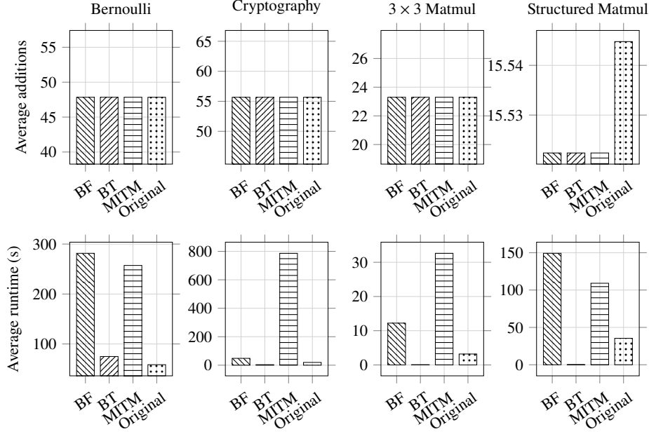
Fig. 28: Average number of additions and average runtime for brute force, sparsity-aware backtracking, meet-in-the-middle, and the original Boyar-Peralta SLP heuristic on the Bernoulli, Cryptography, 3 \times 3 matrix multiplication, and structured matrix multiplication datasets. No preprocessing or postprocessing was applied. Each run was given a maximum wall-clock time of 3 hours per instance and 48 GB of RAM, and averages are computed only over instances for which all methods completed within these limits. The brute-force method is denoted “BF”, the sparsity-aware backtracking method “BT”, the meet-in-the-middle method “MITM”, and “Original” denotes the implementation from [26]. All inputs were supplied via standard input. All experiments were run on a single core of an Intel Xeon E5-2660 v3 CPU.
