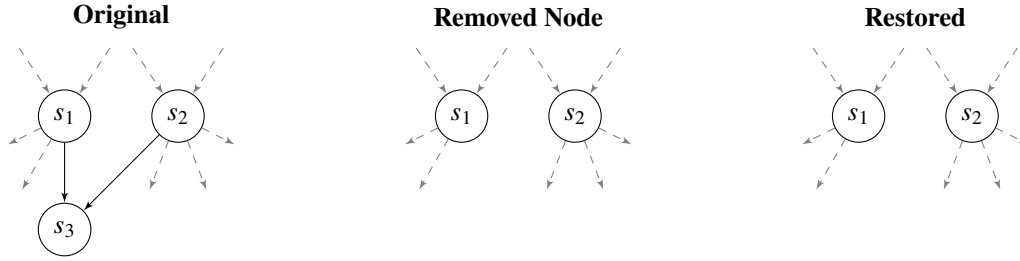
Fig. 38: DAG representation of the second iteration of the rule denoted R2 in [8], when applied through our postprocessing method. The dashed edges represent possible involvement from outside the explicit part of the DAG we're looking at.
