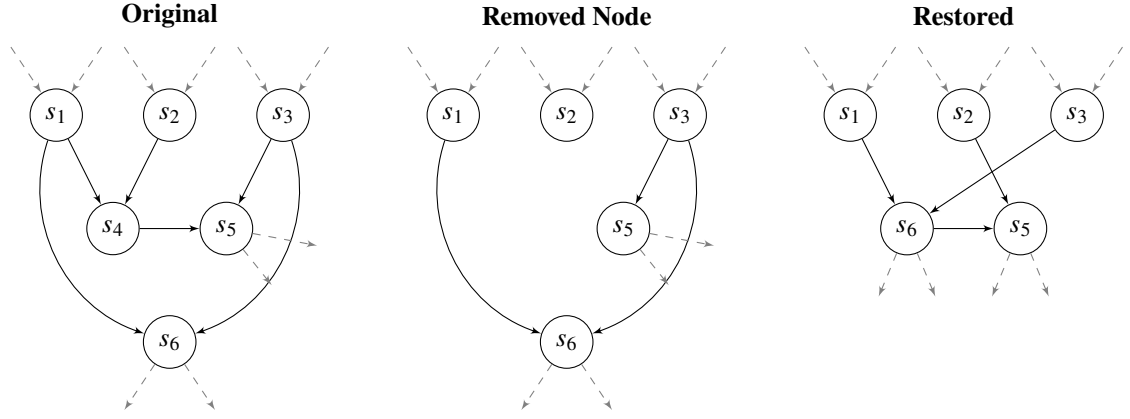
Fig. 39: DAG representation of the rule denoted R3 in [8]. The dashed edges represent possible involvement from outside the explicit part of the DAG we're looking at.
