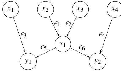
Fig. 5: Variable weighted DAG formulation of addition scheme for G' as it is defined in equation (2.15), but with undetermined \epsilon -weighted edges.
