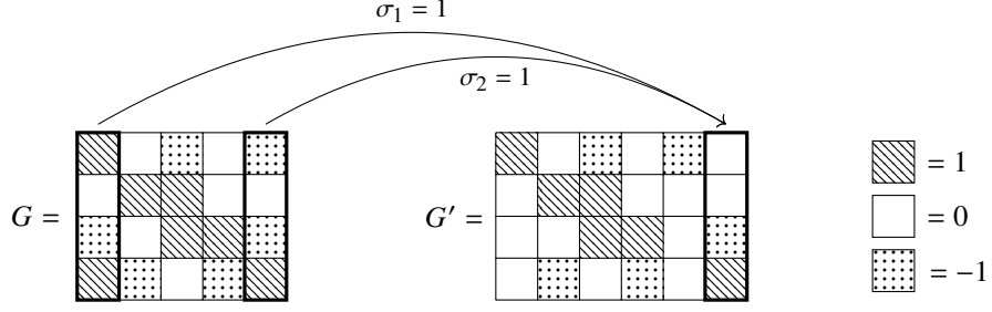
Fig. 15: Depiction of how the vector G_{:,n+1} is constructed, and how the matrix G is augmented, when \sigma = 1 and (j_1, j_2) = (1, 5) .
