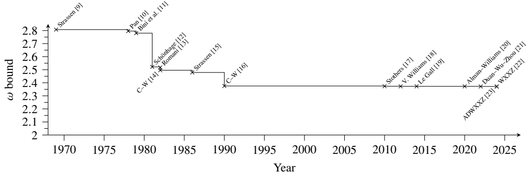
Fig. 1: Progress on the best upper bound on the matrix multiplication exponent \omega , where \omega is such that two n \times n matrices can be multiplied in O(n^\omega) arithmetic operations. Data points are taken from the cited works, the visualization is inspired by [24].
