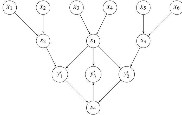
Fig. 6: \mathbb{F}_2 DAG formulation of addition scheme for G' as it is defined in equation (2.17).
