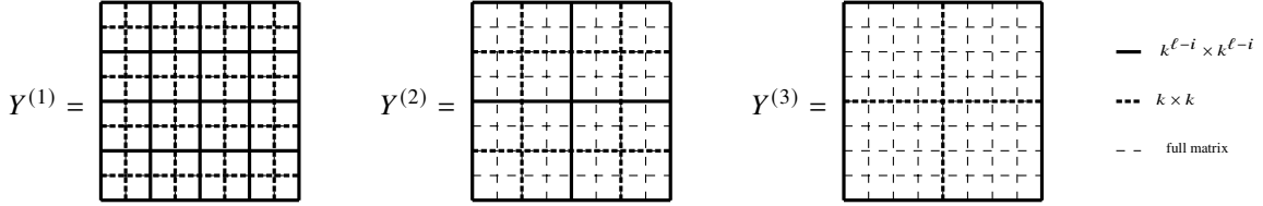
Fig. 9: Illustration of matrices Y^{(1)}, Y^{(2)} , and Y^{(3)} for matrix Y \in \mathbb{F}^{8 \times 8} , that is k = 2 , and \ell = 3 .
