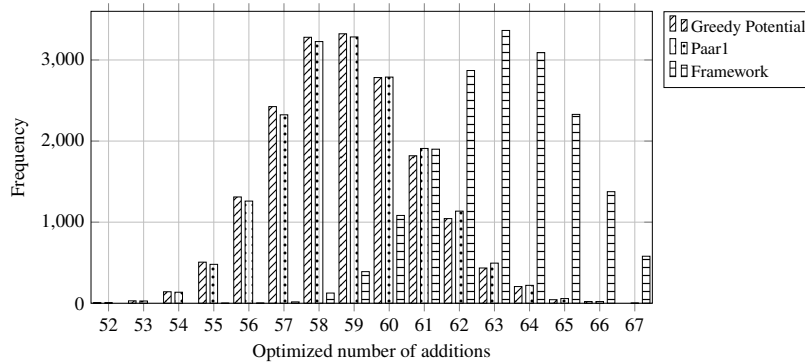
Fig. 35: Frequency distribution of the result of running a 32-thread parallelized solver over the 3 \times 3 dataset with basis-change matrices. The best scheme found for each data point is recorded, together with the corresponding best basis change matrix B_U, B_V, B_W . The framework results were given a time limit of 2.4 seconds per instance, and 128 basis change matrices were used. The greedy-potential and Paar1 methods were run with 500,000 basis change matrices drawn from the set of invertible Bernoulli-random matrices with Bernoulli bias \rho = 0.04 .
