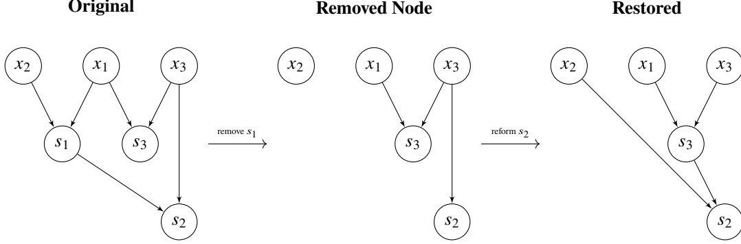
Fig. 22: Illustration of how the swapping orders postprocessing method is a special case of the proposed postprocessing scheme. The shown DAG might be part of a larger DAG, but as long as s_1 is used only in forming s_2 the shown reduction holds. Note that we could also form x_2 = s_2 + s_3 , giving a new connected DAG, but this would not preserve the previous topological ordering, and is hence not considered by the described postprocessing approach.
