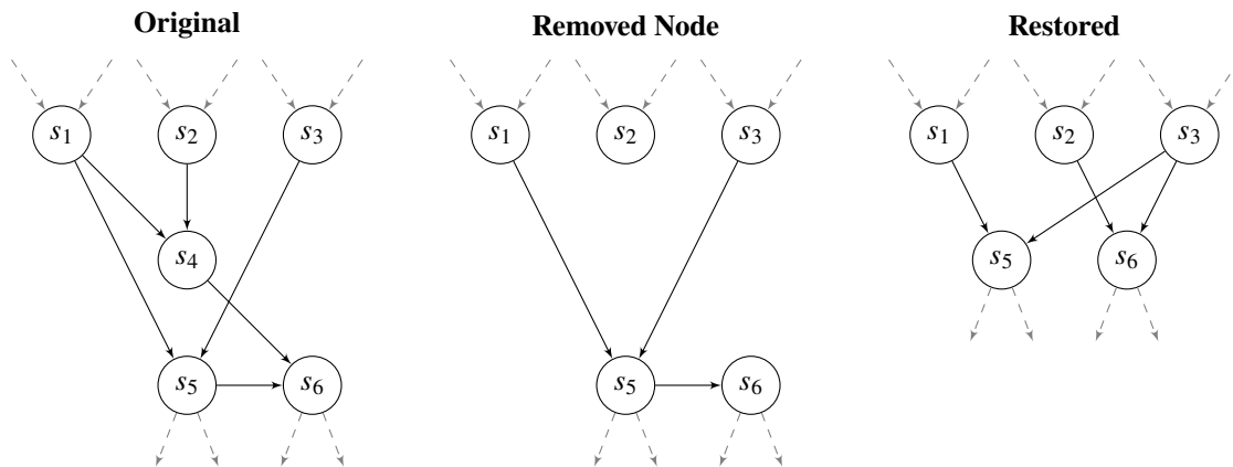
Fig. 43: DAG representation of the rule denoted R9 in [8]. The dashed edges represent possible involvement from outside the explicit part of the DAG we're looking at.
