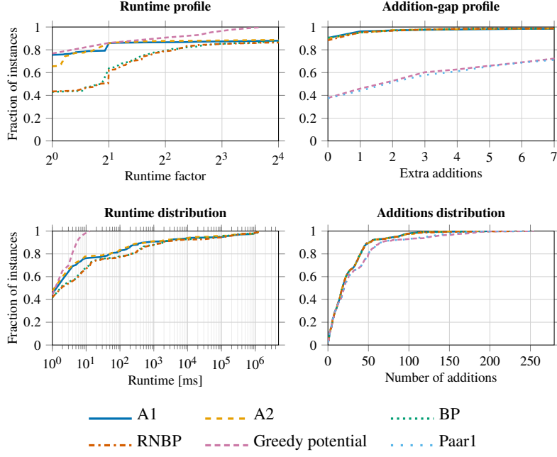
Fig. 31: Comparison of the six heuristics on the structured matrix multiplication dataset. We remark that the Paar1 heuristic took 0 milliseconds (we round to nearest millisecond) on most data points, hence its missing representation on the runtime plots. No preprocessing or postprocessing was applied. All instances were run on a single core on an Intel Xeon E5-2660 v3 CPU model, and the time limit given was 1200 seconds per instance of SLP we solve - hence the sharp cutoff of the runtime at 1200000 milliseconds.
