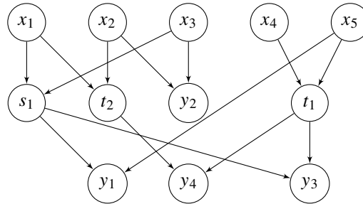
Fig. 24: Result of back-substituting the addition scheme for S_o , and S_i into the original addition scheme. Note that in the original addition scheme we had s_2, s_3 \in B' , hence why they were removed.
