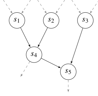
Fig. 20: Illustration of the construction of the subgraph with root s_5 and \ell = 3 according to the breadth-first search described. The dashed gray edges show that this is possibly part of a larger addition scheme, but the breadth first search only considers s_1, s_2, s_3, s_4 , and s_5 .
