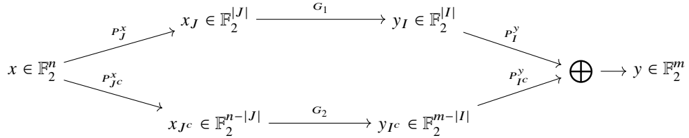
Fig. 12: Illustration of computing an addition scheme of a separable instance of Problem 2.1 induced by the matrix G , by decomposing into instances of Problem 2.1 induced by G_1 and G_2 .
