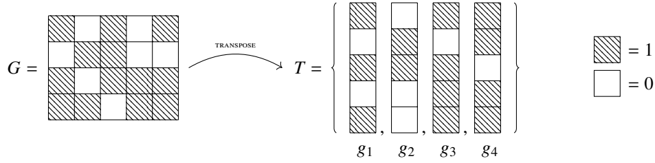
Fig. 16: Illustration of how the set of target vectors described in Problem 2.1 is constructed. In this example, we work over \mathbb{F}_2 , in general the - entries would simply indicate nonzero entries.
