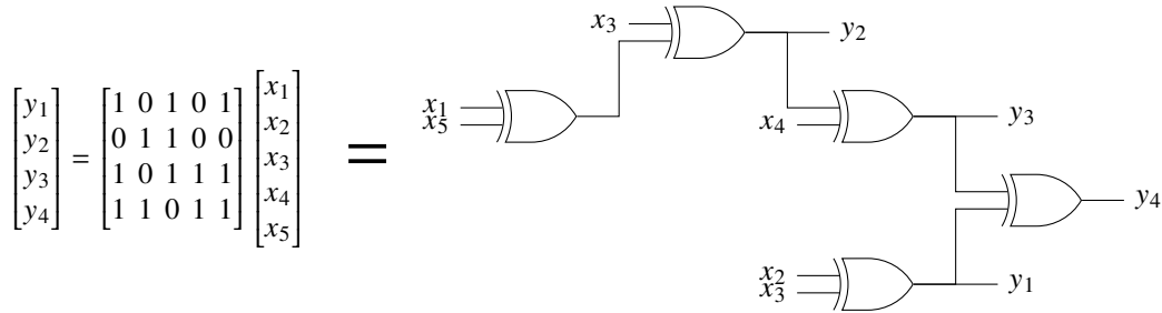
Fig. 10: Equivalence between XOR circuit and addition scheme. The addition scheme represented here is the same as for the example used in Section 2.3.1.
