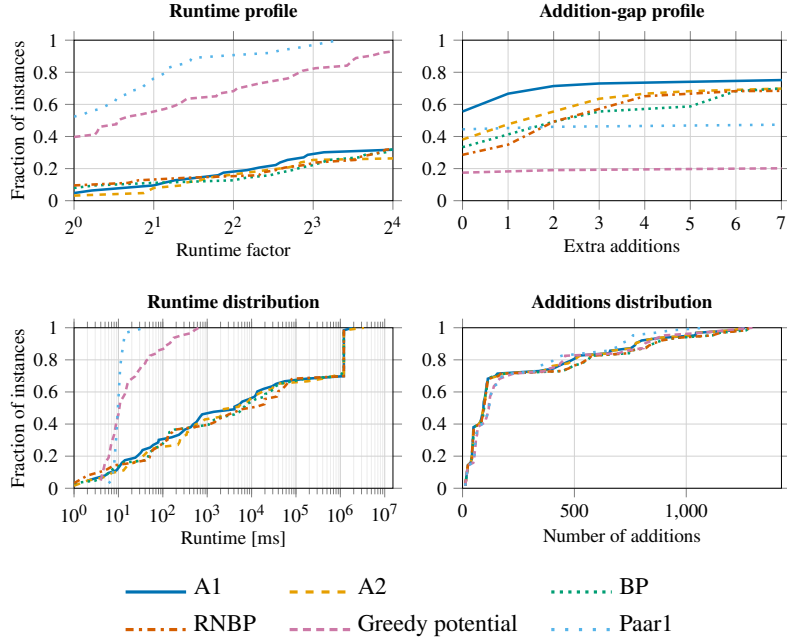
Fig. 30: Comparison of the six heuristics on the Crypt dataset. The runtime-profile and addition-profile show the fraction of instances solved within a given factor of the fastest method and best addition scheme respectively, on the same instance. No preprocessing or postprocessing was applied. All instances were run on a single core on an Intel Xeon E5-2660 v3 CPU model, and the time limit given was 1200 seconds per instance of SLP we solve - hence the sharp cutoff of the runtime at 1200000 milliseconds.
