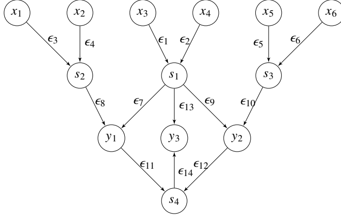
Fig. 7: DAG formulation of addition scheme for G' as it is defined in equation (2.17), but with undetermined \epsilon -weighted edges.
