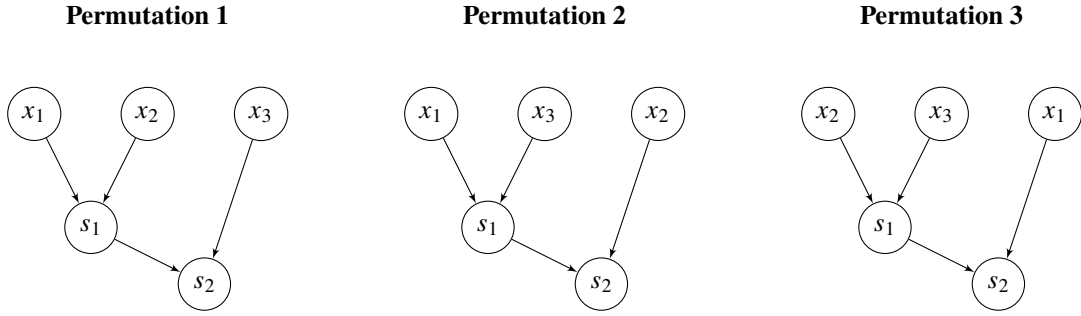
Fig. 21: Example of permutations of processing subgraph from Figure 20 to reduce the number of additions required to compute the addition scheme. Note that the variable s_2 is computed the same way, independent of the way the leaves are permuted, so if one of s_1 = x_1 + x_2 , s_1 = x_1 + x_3 , and s_1 = x_2 + x_3 is a target vector, or is used elsewhere in the addition scheme, then the right permutation of the leaves might save us an addition. This illustration was inspired by Figure 1 in [39].
