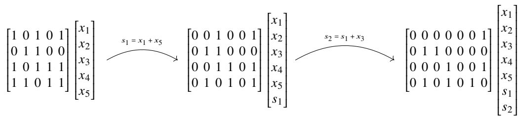
Fig. 14: Matrix form of Paar1 on the example instance of Problem 2.1.
