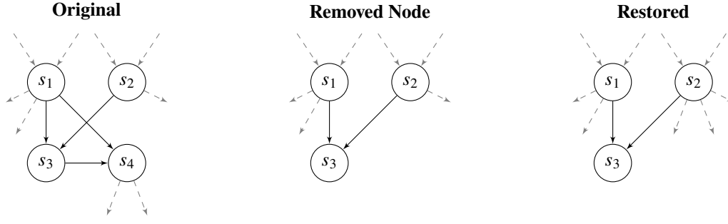
Fig. 37: DAG representation of the first iteration of the rule denoted R2 in [8], when applied through our postprocessing method. The dashed edges represent possible involvement from outside the explicit part of the DAG we're looking at.
