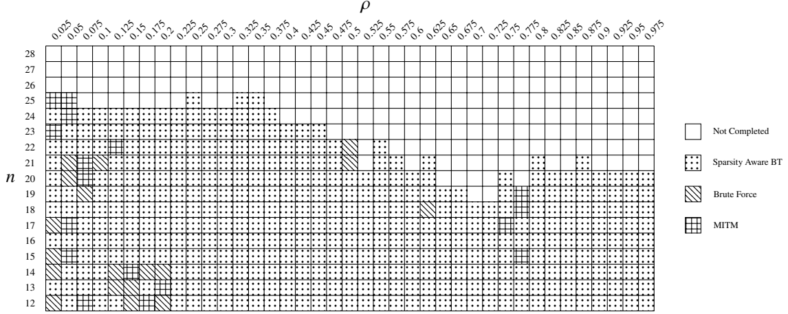
Fig. 18: Map over the best performing REACHABLE strategy out of Algorithms 4–6 used in the Boyar-Peralta heuristic on the Bernoulli random matrices from the dataset described in Section 3.4. All instances were run on a single core, on a XeonE5_2660v3 CPU, and were terminated if it required more than 3 hours to complete. If no method terminated within the timelimit we mark the square as Not Completed .
