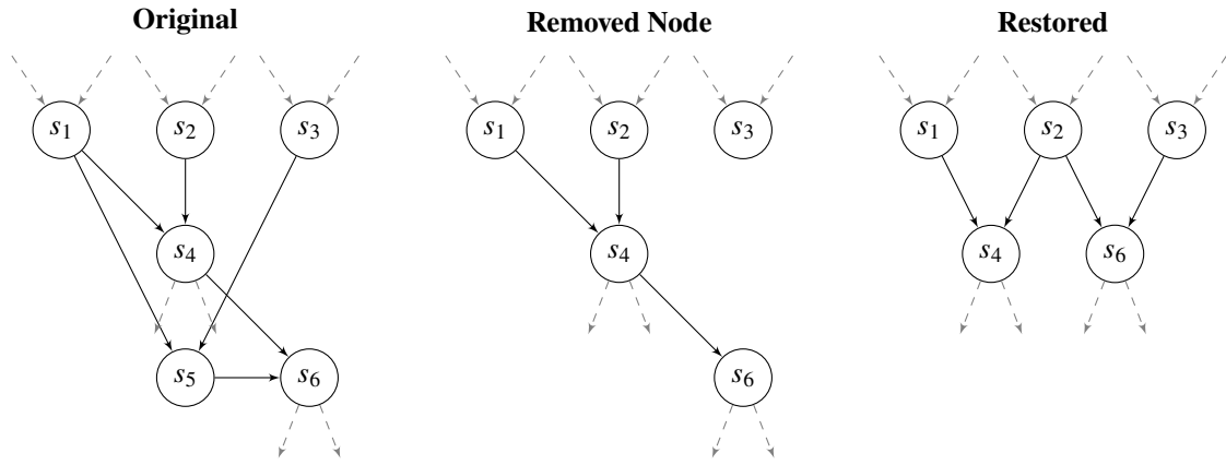
Fig. 44: DAG representation of the rule denoted R10 in [8]. The dashed edges represent possible involvement from outside the explicit part of the DAG we're looking at.
