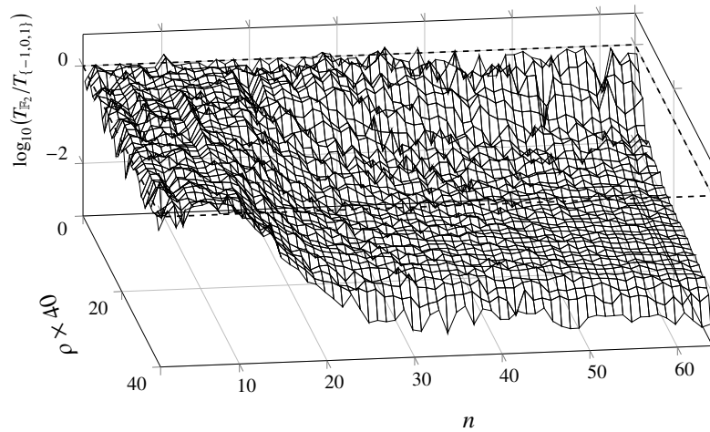
Fig. 27: Surface plot comparing the time, T_{\mathbb{F}_2} , required to compute each \mathbb{F}_2 scheme of the dataset in Section 3.4.1 to the time, T_{\{-1,0,1\}} , required to compute each of the \{-1, 0, 1\} schemes of the same dataset. All instances were run on a single core on an Intel Xeon E5-2660 v3 CPU model.
