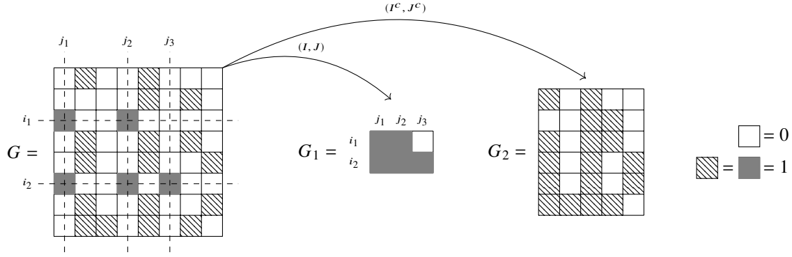
Fig. 11: Illustration of separability of matrix G into two distinct smaller matrices G_1 and G_2 from index sets I = \{i_1, i_2\} and J = \{j_1, j_2, j_3\} .
