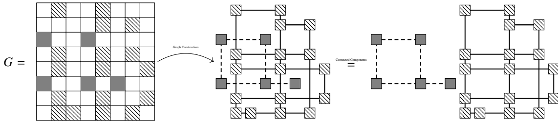
Fig. 13: Constructing the graph from the corresponding matrix and finding the connected components of the corresponding graph. Here, \blacksquare denotes the (I, J) -indexed entries, \square denotes the non- (I, J) entries, and \square denotes zero entries. We remark that the example matrix G is the same used in Figure 11.
