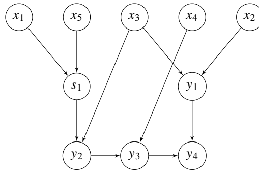
Fig. 3: Directed acyclic graph representation of the addition scheme for the matrix in equation (2.11) also illustrated in equations (2.12) and (2.13). The ordering of x_1, \dots, x_5 is chosen so as to minimize edge overlaps.
