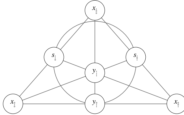
Fig. 19: Representation of the union over all possible addition schemes in DAG formulation, such that there are 3 inputs x_1, x_2 , and x_3 , and two outputs, namely y_1 = x_1 + x_2 + x_3 , and y_2 = x_2 + x_3 . Any two nodes on the same line or circle XOR to the third.
