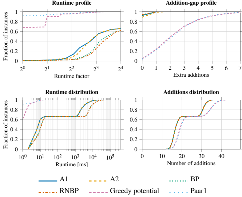
Fig. 29: Comparison of the six heuristics on the 3 \times 3 matrix multiplication dataset, see Section 3.1. The runtime-profile and addition-profile show the fraction of instances solved within a given factor of the fastest method and best addition scheme respectively, on the same instance. No preprocessing or postprocessing was applied. 32 Bernoulli-random invertible basis change matrices drawn with Bernoulli bias parameter \rho = 0.04 , were used for each data point, and applied as detailed in Section 3.1.1. All instances were run on a single core on an Intel Xeon E5-2660 v3 CPU model, and the time limit given was 1200 seconds per instance of SLP we solve.
