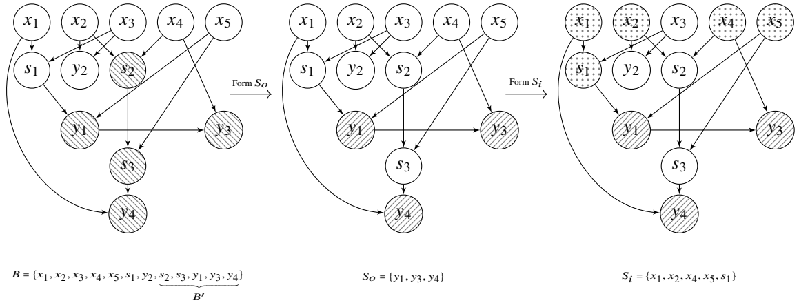
Fig. 23: Illustration of how a certain slice B' , illustrated with \odot , of an addition scheme B for the example instance of Problem 2.1 introduced in Section 2.3.1 gives rise to the sets S_o , illustrated with \oslash , and S_i , illustrated with \odot .
