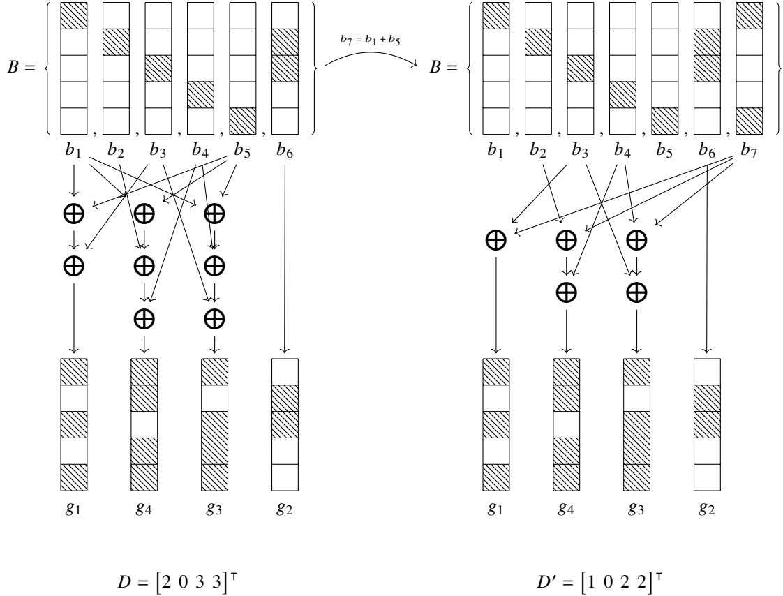
Fig. 17: We continue the example from Figure 16, working over \mathbb{F}_2^5 , and show the effect of adding a new element b_{|B|+1} to B on the distance vector D . The illustration shows the second step of the BP heuristic, the first step added b_6 = b_2 + b_3 to our set B . Each target vector is calculated independently, and each distance entry D_i corresponds exactly to the number of \oplus above it. Note that the target vectors g_1, \dots, g_4 are not ordered according to their index in the illustration, this is simply to avoid too much clutter.
