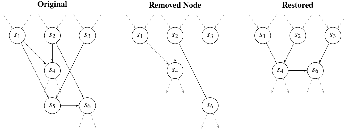
Fig. 40: DAG representation of the rule denoted R5 in [8]. The dashed edges represent possible involvement from outside the explicit part of the DAG we're looking at.
