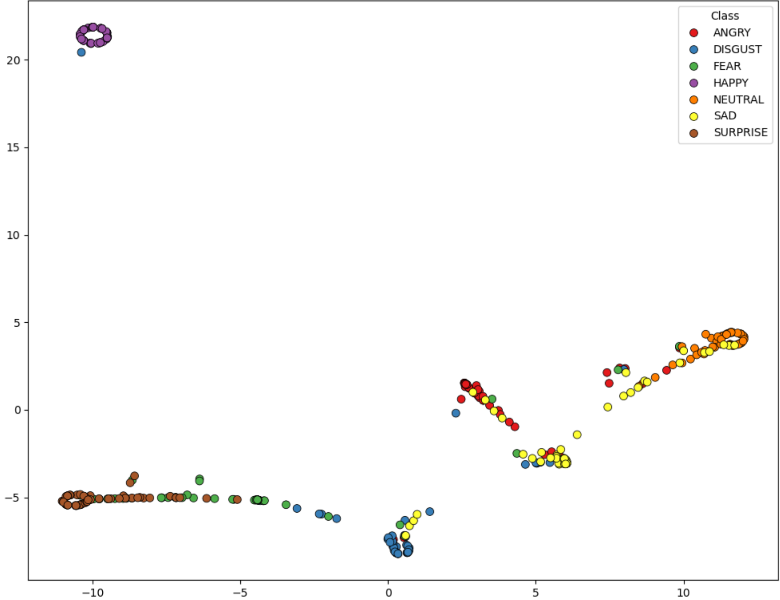
t-SNE Visualization of Features with perplexity 50
