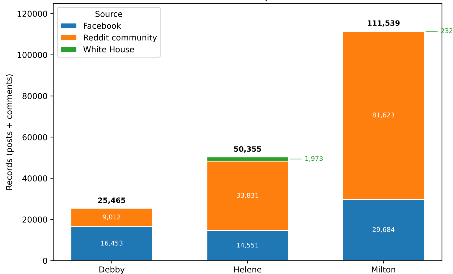
Dataset overview — records by source and hurricane
