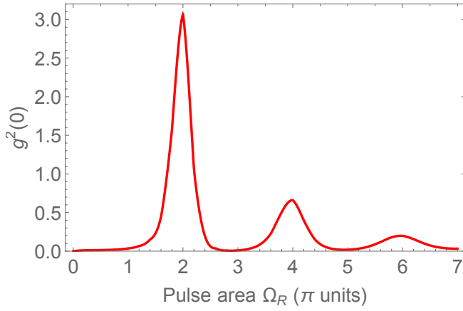
FIG. 3. Second-order correlation function at zero delay, g^{(2)}(0) , as a function of the pump pulse area.
