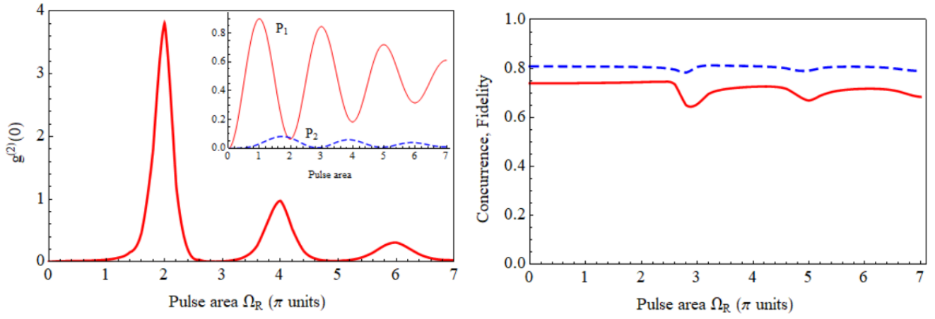
FIG. 2. (Left) Second-order correlation function at zero delay, g^{(2)}(0) , as a function of the pump pulse area. Inset: Probabilities of the one-photon, P_1 (solid), and two-photon, P_2 (dashed), emission as functions of the pump pulse area. (Right) Concurrence (solid) of the emitted two-photon polarization state and fidelity (dashed) to the Bell state |\Phi^+\rangle as a function of the pump pulse area.
