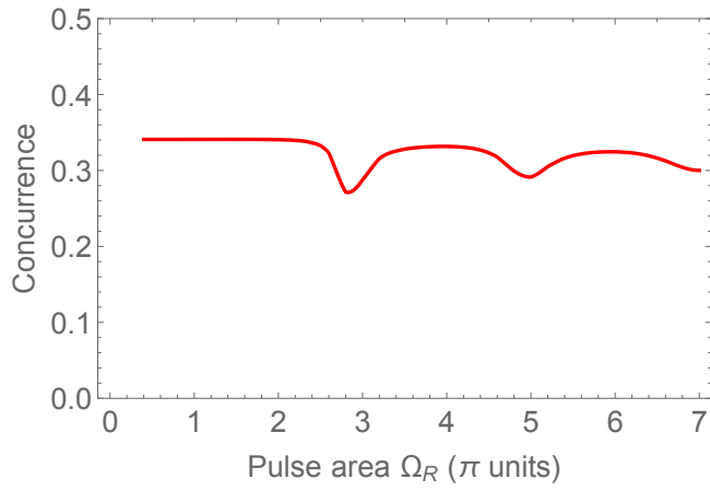
FIG. 4. concurrence
