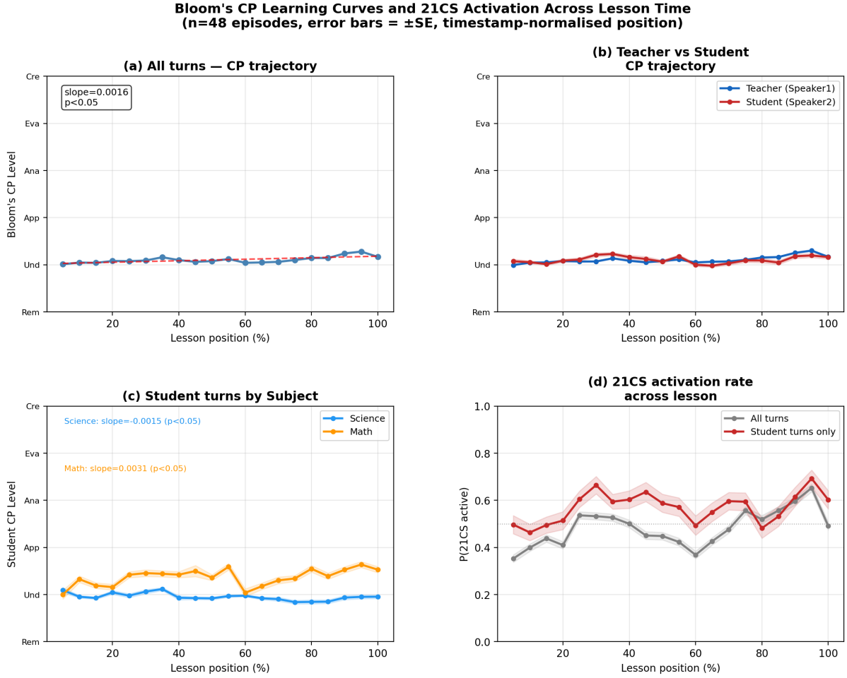
Figure 5: Bloom's Cognitive Process (CP) trajectory and 21CS activation across lesson time ( n=48 episodes, B=20 bins of 5% width, error bars = \pm SE , Eqs. 52-58). Panel (a): all-turns CP trajectory (Eq. 54-56); slope \hat{\beta}=0.0016 ( p < 0.05 ) confirms a statistically significant but practically negligible positive trend, the classroom operates near Understanding level ( CP \approx 2 ) throughout. Panel (b): teacher (Speaker1) and student (Speaker2) CP trajectories are near-identical, confirming a uniform cognitive register regardless of speaker. Panel (c): student-only trajectories by subject (Eq. 59); Math shows a rising trend ( \hat{\beta}=+0.0034 , p < 0.05 ) while Science shows a slight decline ( \hat{\beta}=-0.0013 , p < 0.05 ), reflecting the hierarchical structure of mathematics instruction. Panel (d): 21CS activation rate across lesson (Eq. 58); student turns begin near \hat{P}=0.47 , rise to \hat{P} \approx 0.60 by the 25th percentile, dip near the 60th percentile at the typical Teaching-Assessment phase transition, then recover to \hat{P} \approx 0.65 at lesson end.
