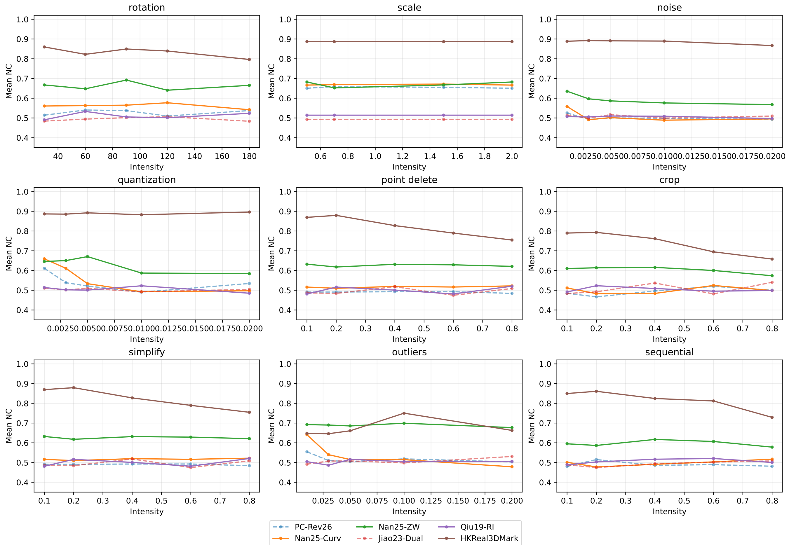
Hong Kong oblique-photogrammetry watermark baselines (seed=2026)
