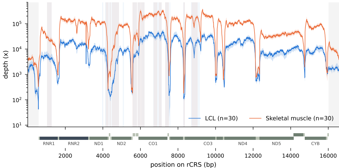
Figure 1 chrM coverage landscape shaded: control region (grey) and NUMT-affected regions (cohort colour)
