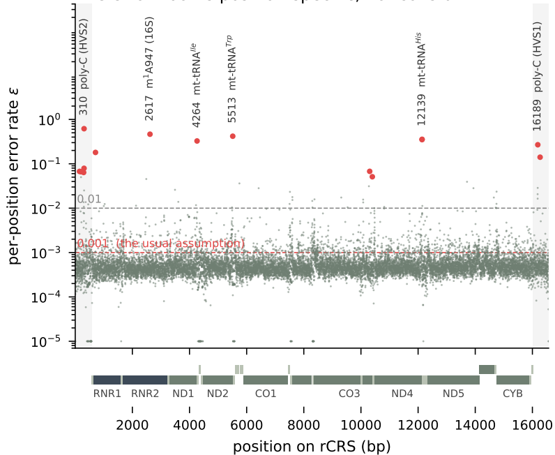
The error floor is position-specific, not constant
