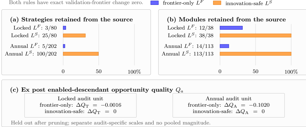
Figure 4: Financial safety-compression trade-off for the current stepwise endpoints. Panels (a)–(b) report exact retained fractions of each fixed source library and module closure. Panel (c) reports \Delta Q_a = Q_a(L') - Q_a(L) , the held-out change in the best enabled descendant’s audit-specific opportunity quality; the two audit units are not pooled. Both rules preserve the validation frontier, but only the safe rule preserves closure and Q_a . The displayed Q_a values are rendered audit decimals and are not pruning inputs. Table 4 adds the HiGHS-reported minimum-cardinality and minimum-weight comparisons.
