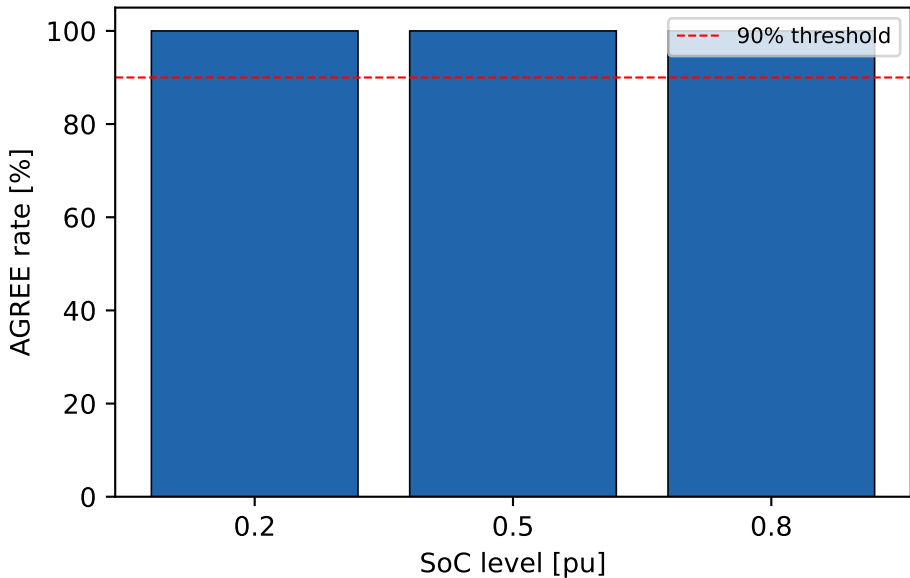
TR-68: BESS AGREE rate by SoC level
