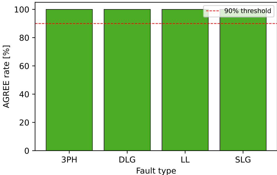
TR-68: BESS AGREE rate by fault type
