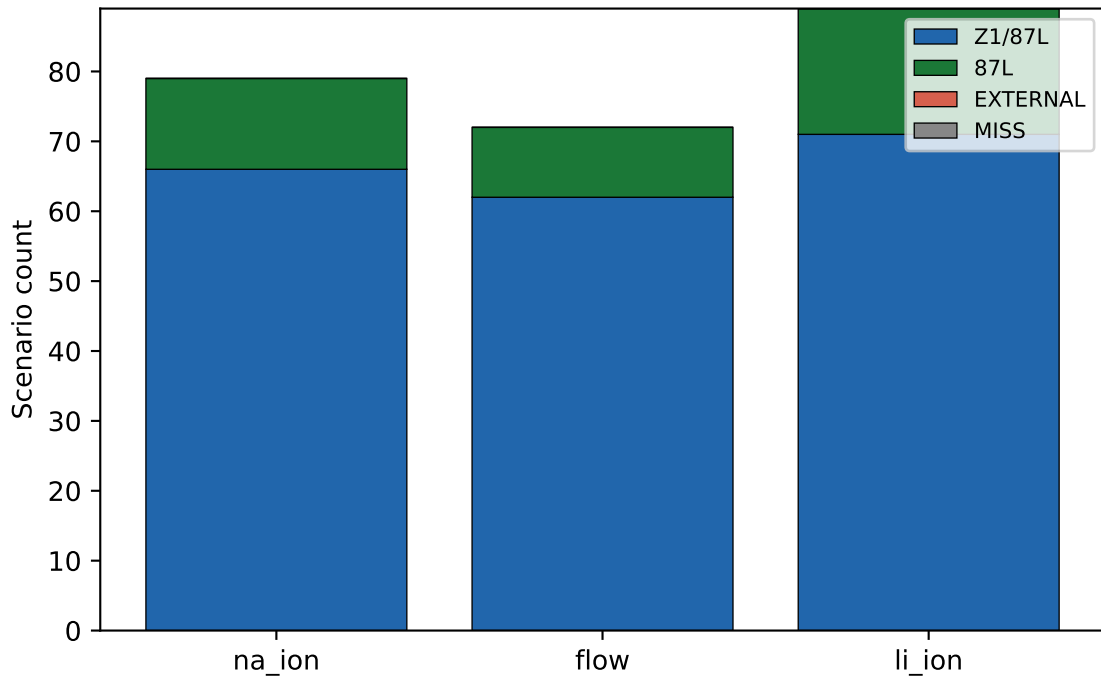
TR-68: Protection outcome distribution by chemistry
