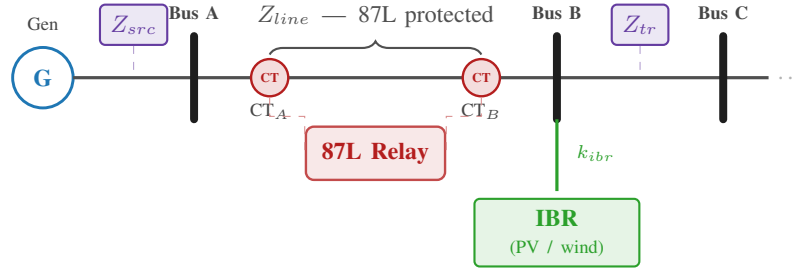
Fig. 1. Study network. The 87L relay receives differential current from CT_A and CT_B via IEC 61850 sampled values. IBR at Bus B limits fault current to k_{ibr} pu. Fault location F (internal scenarios) is at line mid-point.
