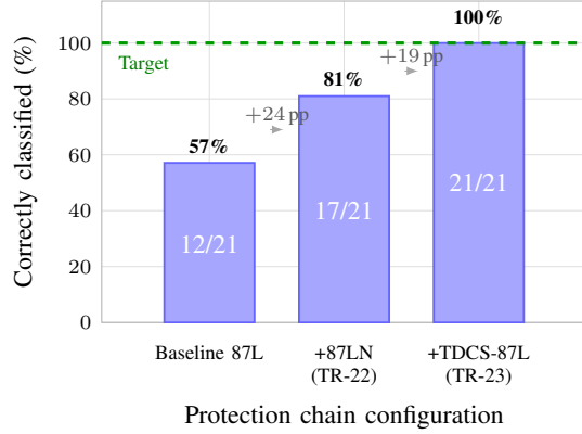
Fig. 7. Cumulative detection accuracy as IBR-adaptive elements are added. 87LN0 recovers five earthed SLG faults; TDCS-87L closes the four symmetric 3PH fault gaps. All 21/21 scenarios are correctly classified by the combined chain.
