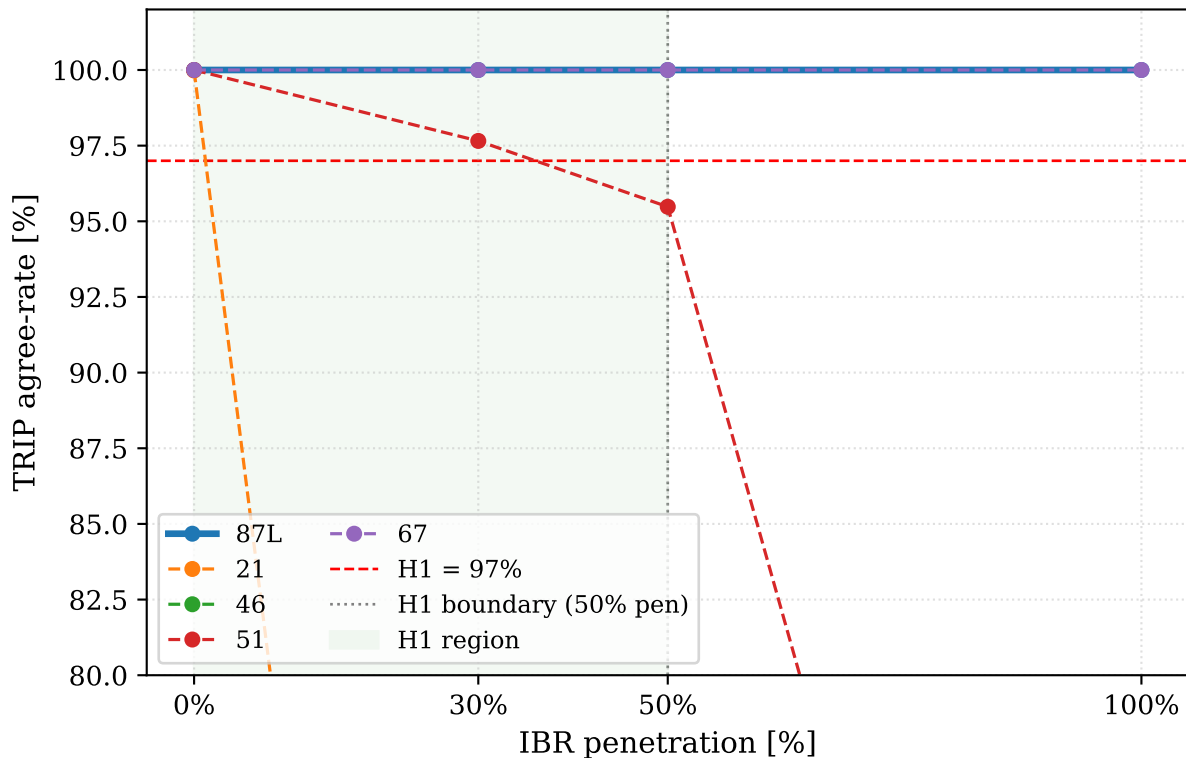
Agree-rate vs IBR penetration IEEE 118-bus, N = 50,000 LHS trials
