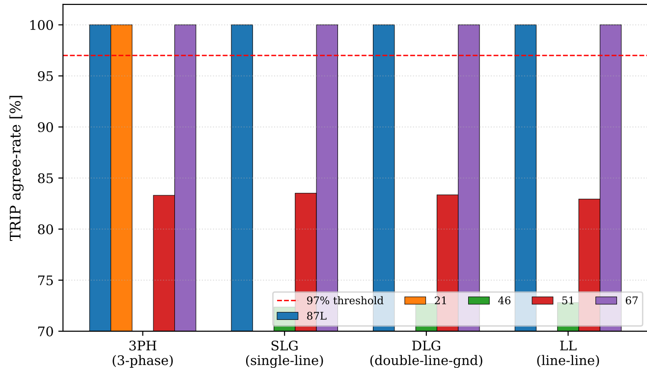
Agree-rate by fault type and protection element IEEE 118-bus, N = 50,000 LHS trials
