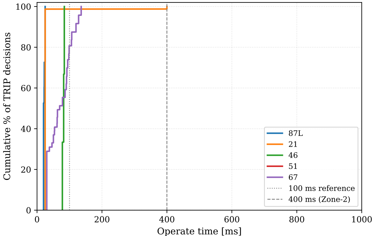
Operate-time CDF (TRIP decisions only) IEEE 118-bus, N = 50,000 LHS trials
