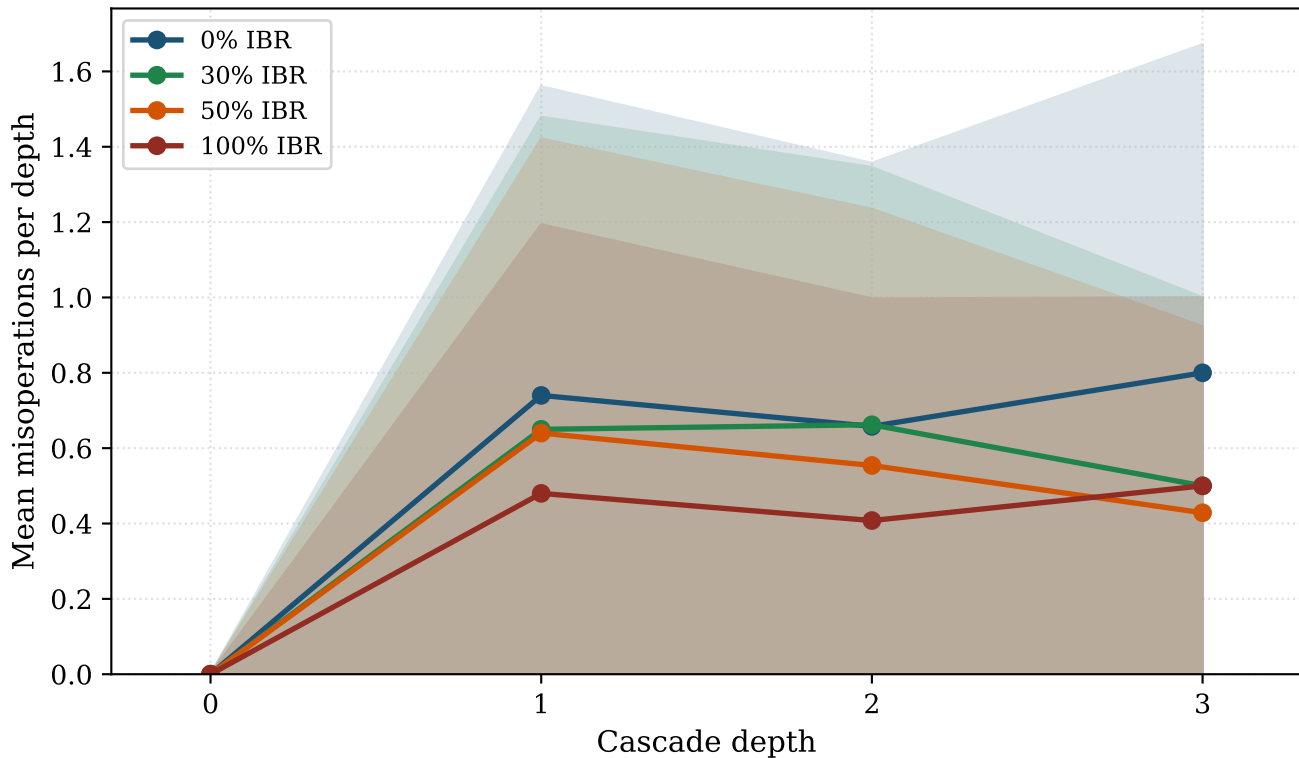
SAMBP misoperation count vs cascade depth Mean \pm 1\sigma across 100 N-2 scenarios
